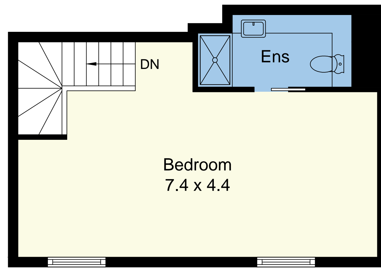
FIRST FLOOR
