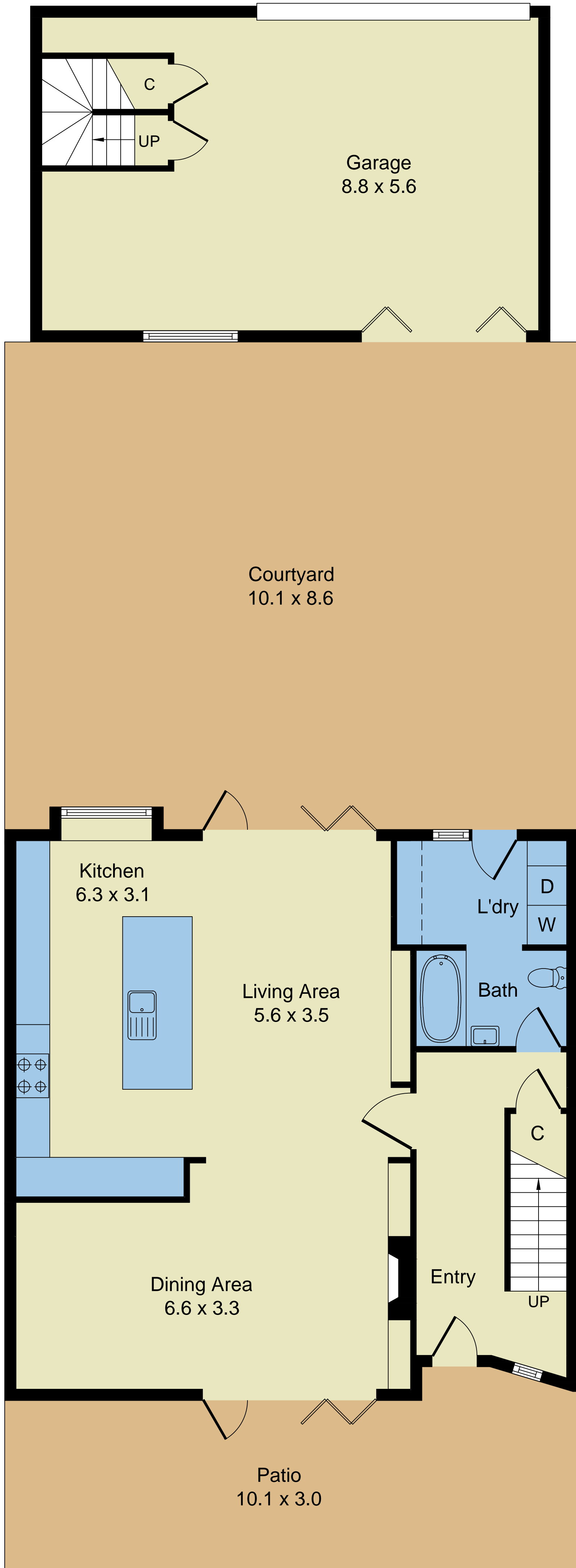
GROUND FLOOR
