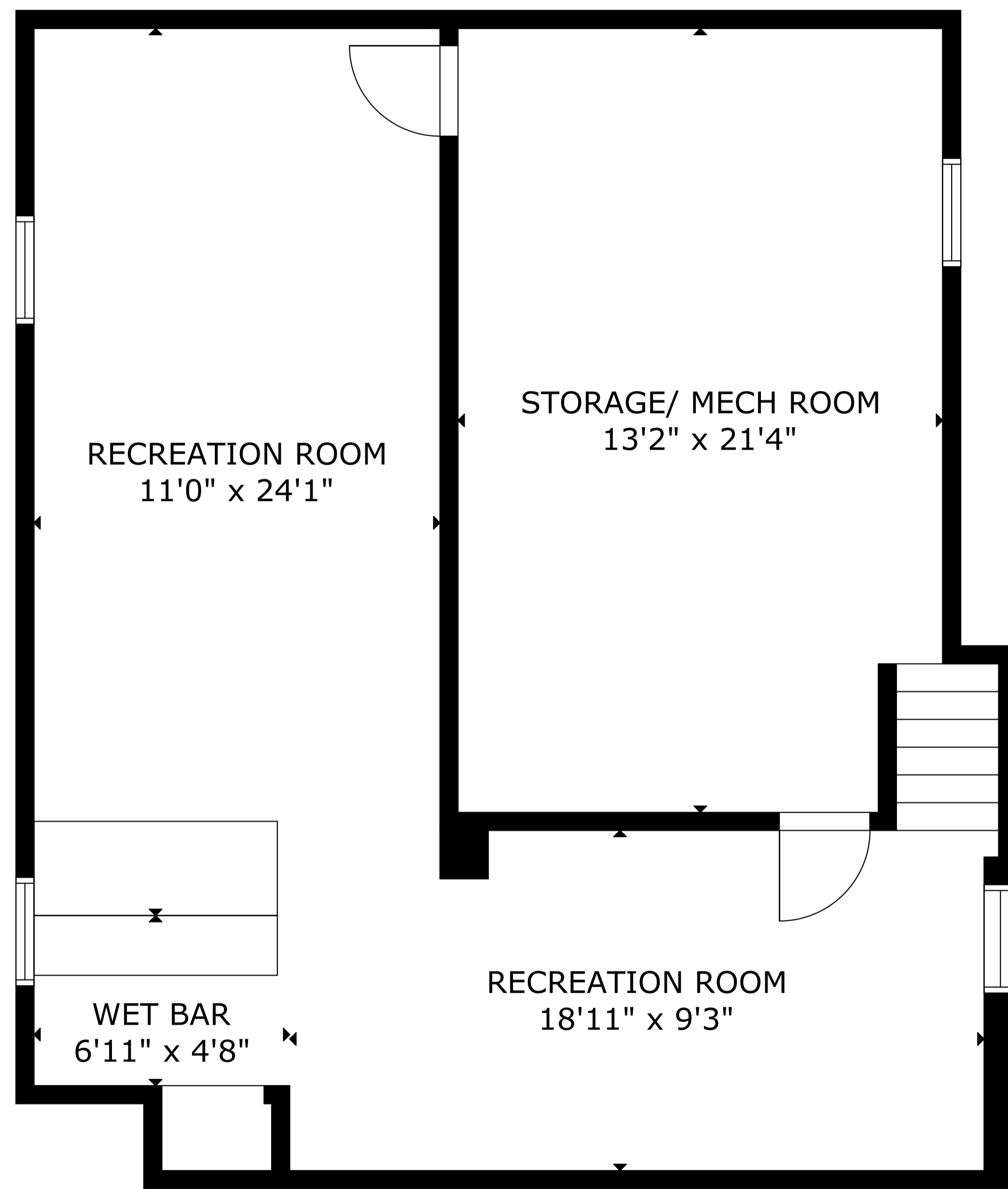
BASEMENT
