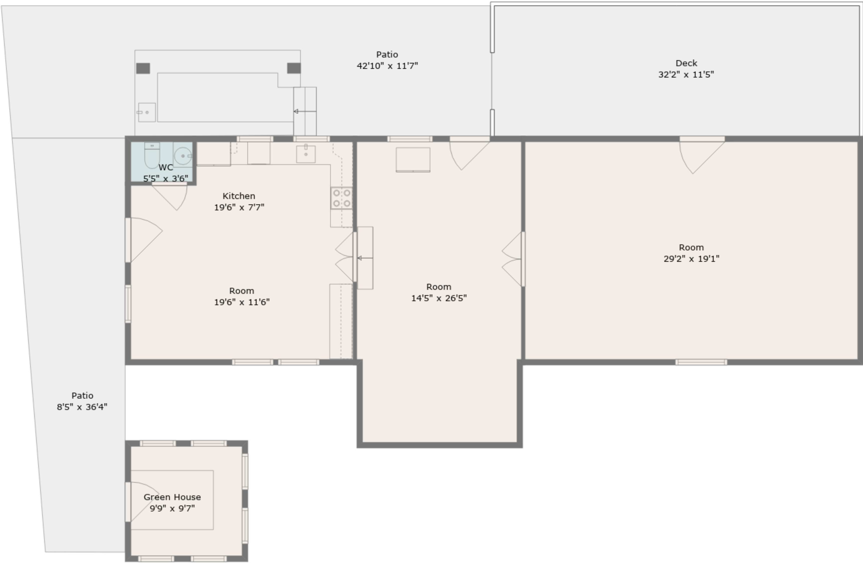
Floor 1
