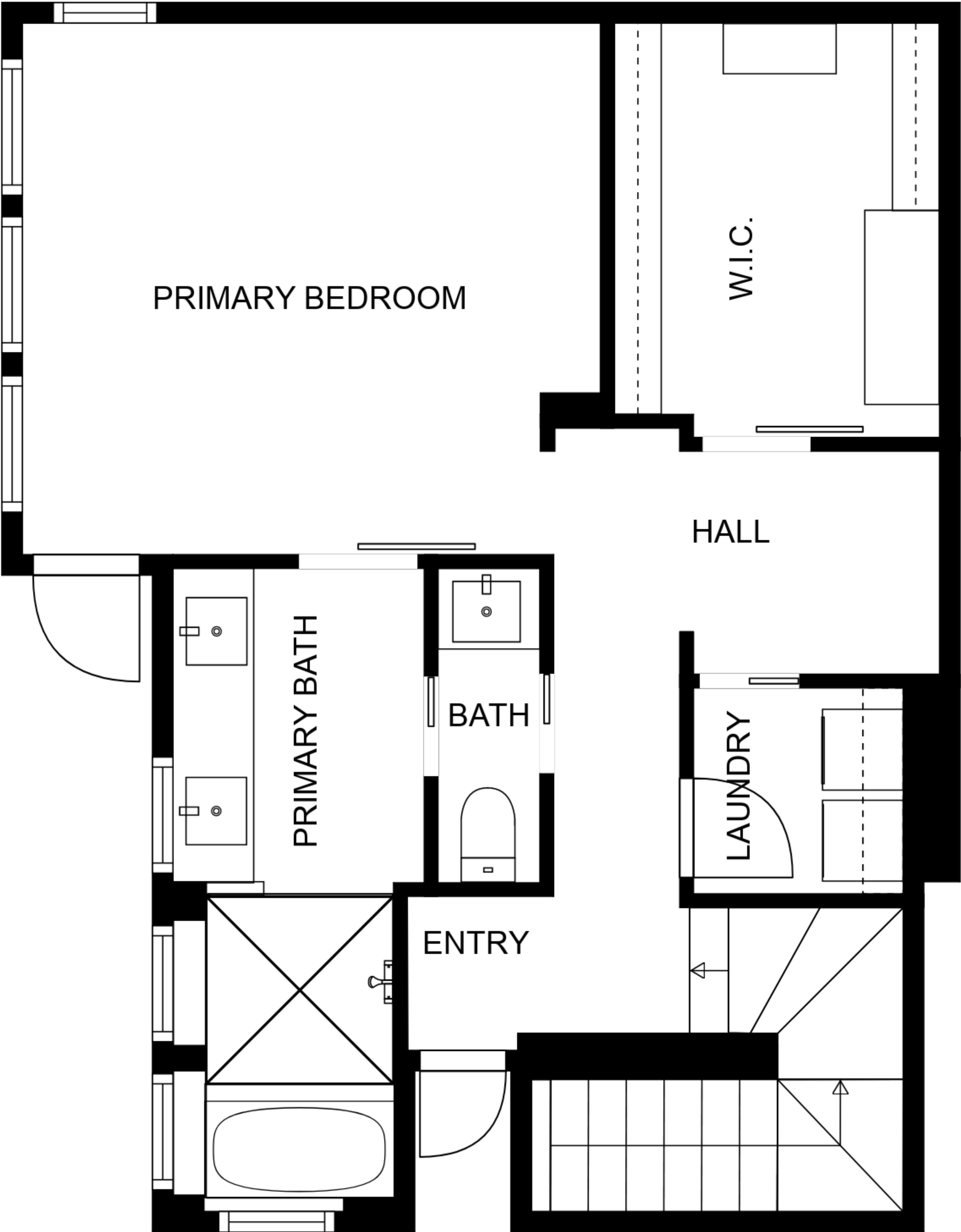
FLOOR 3
