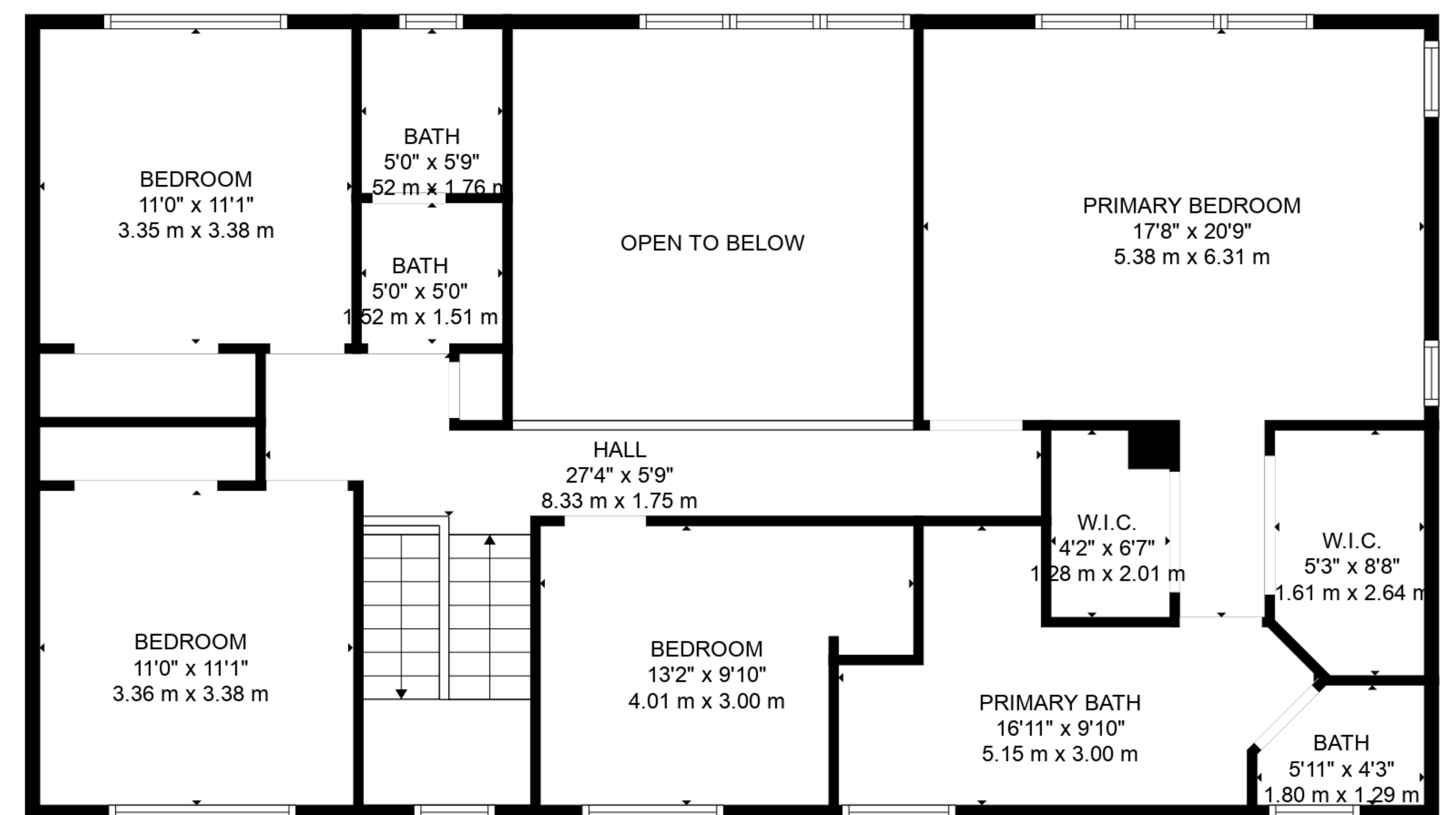
FLOOR 2
