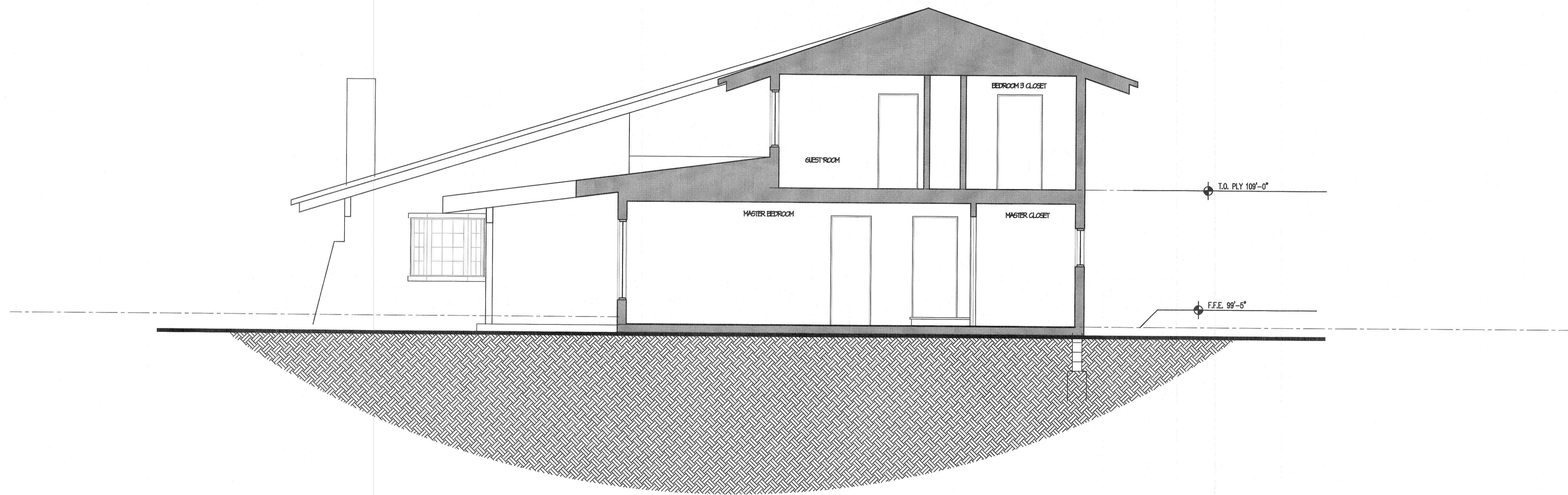
1 PROPOSED SECTION A4.2 1/4" = 1'
