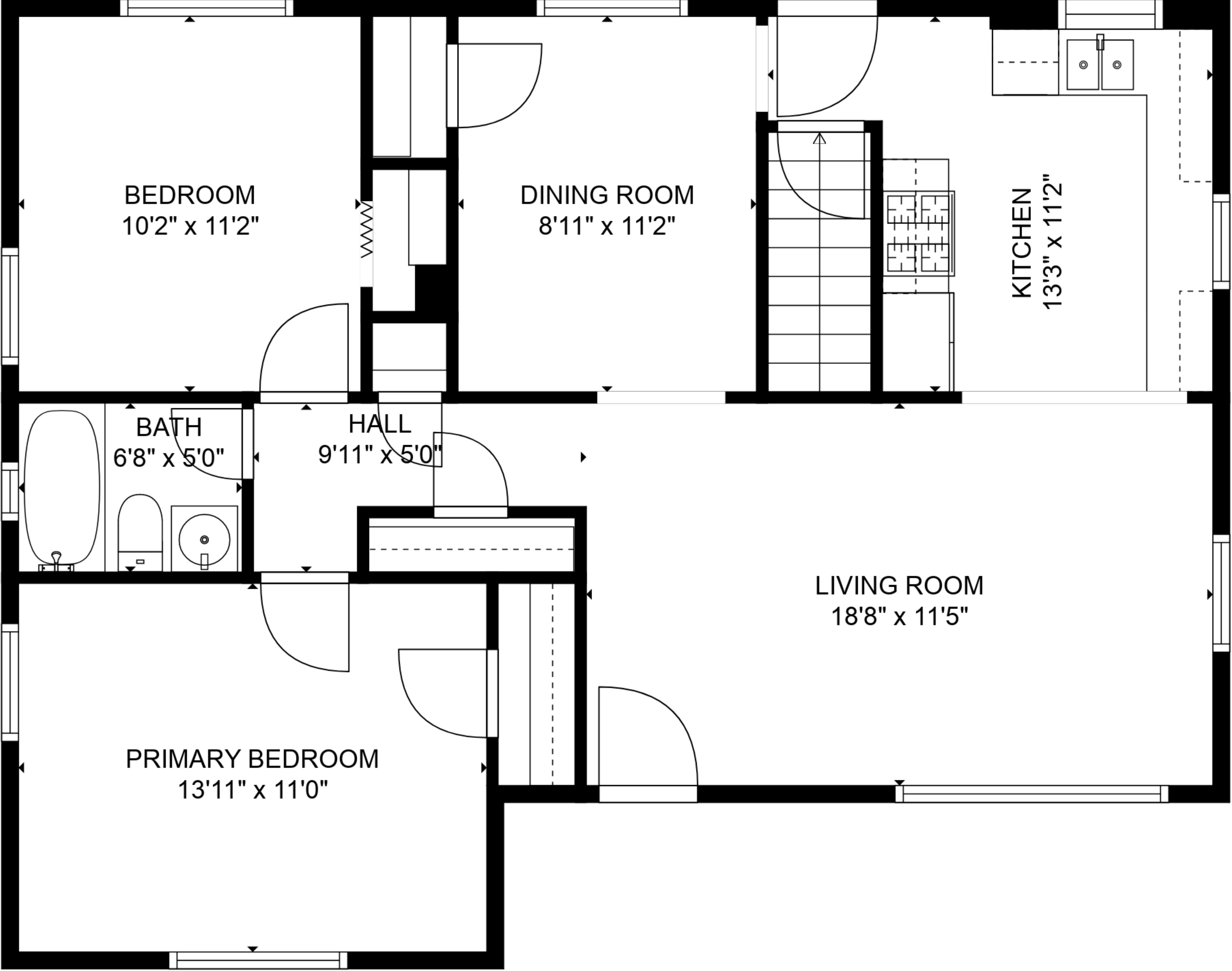
FLOOR 2
