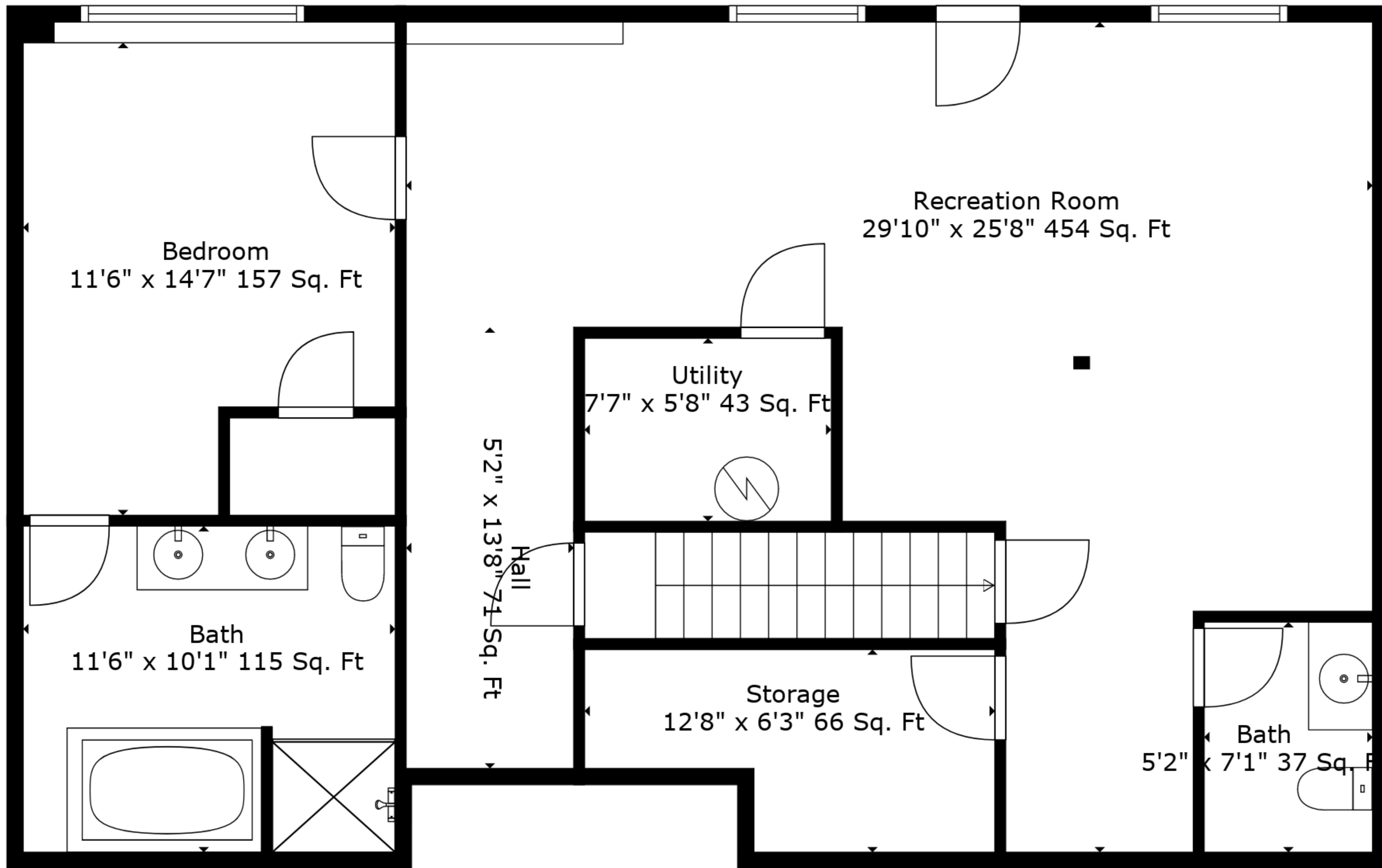
Floor 1
