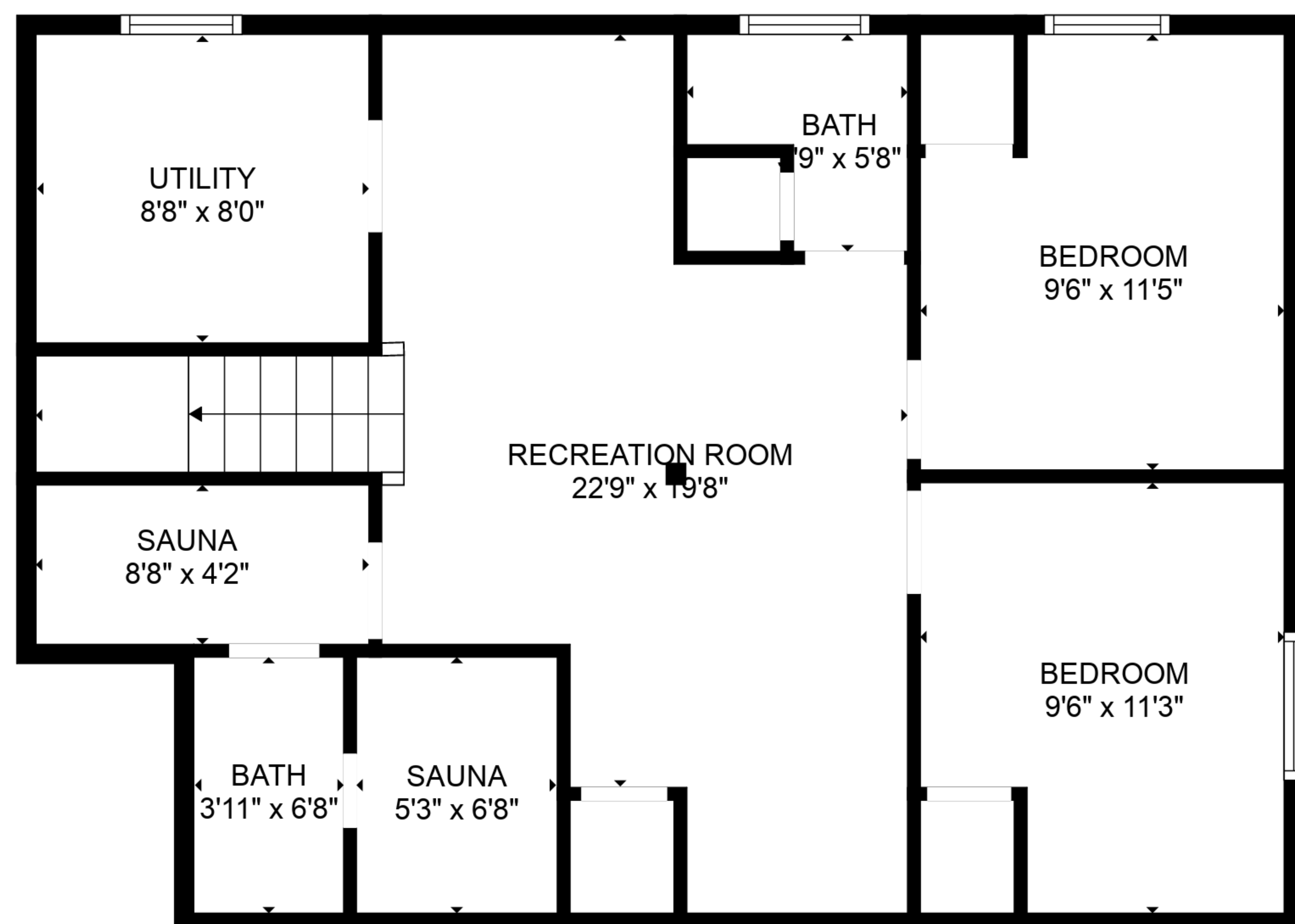
FLOOR 2
