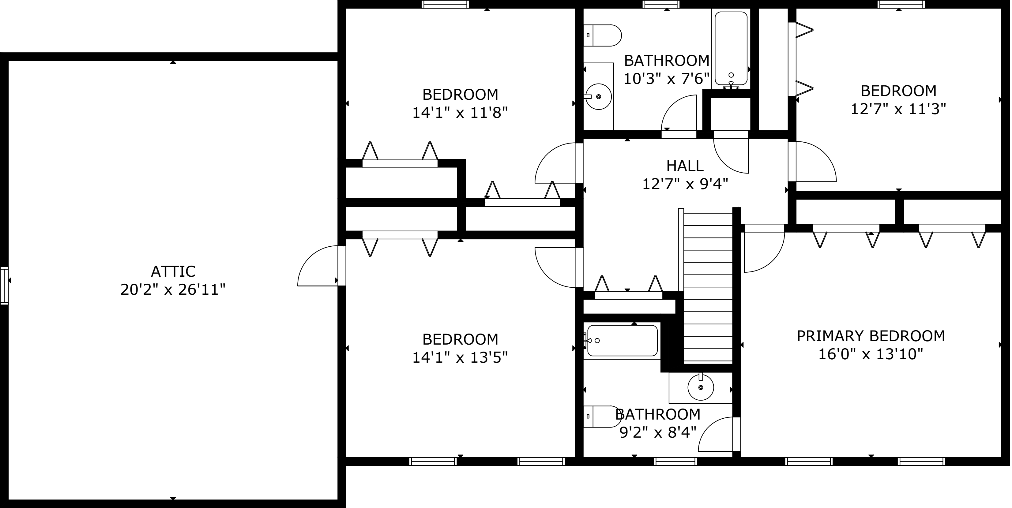
UPPER LEVEL 1
