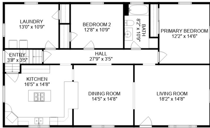
MAIN FLOOR
