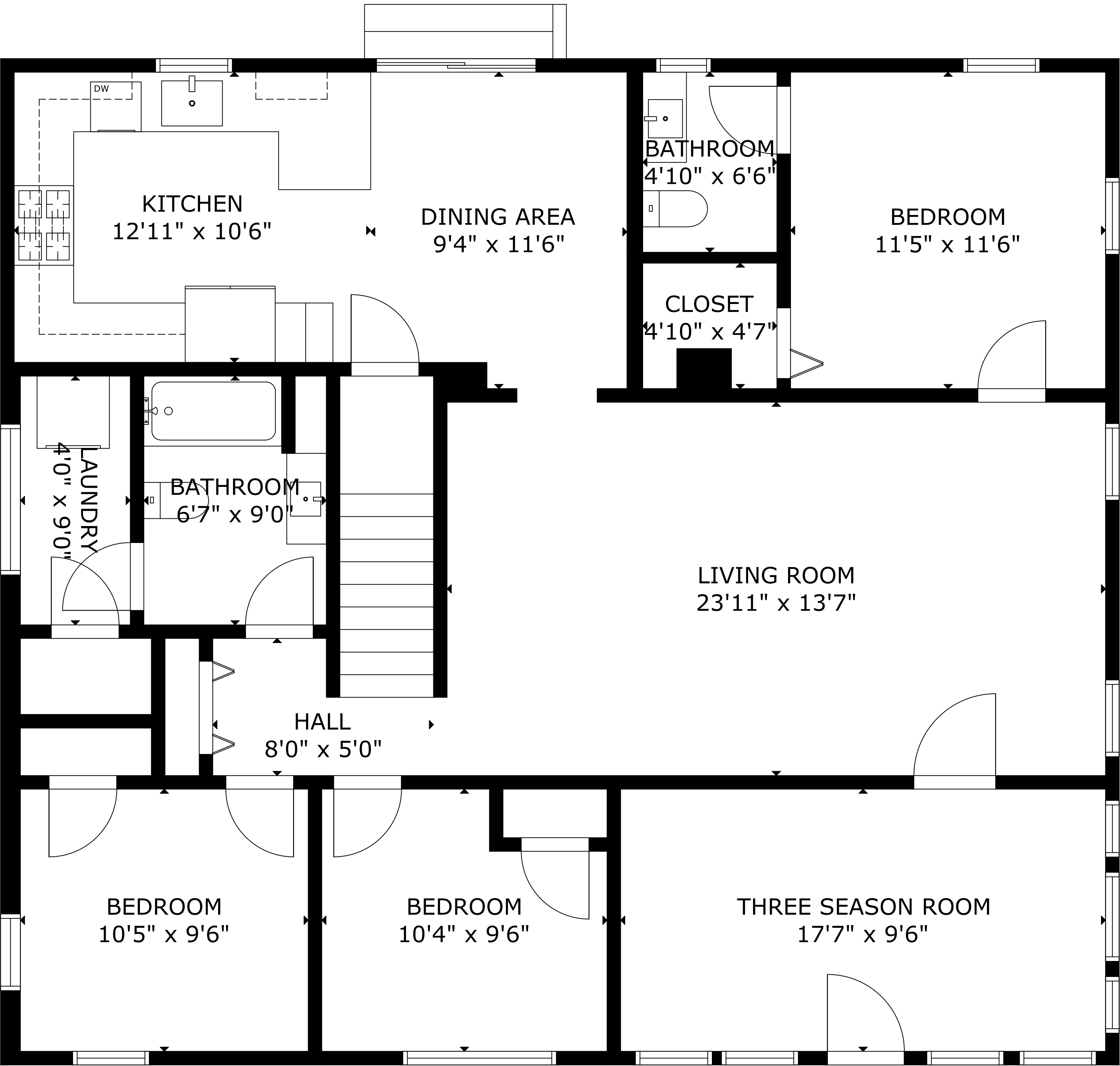
FLOOR 1
