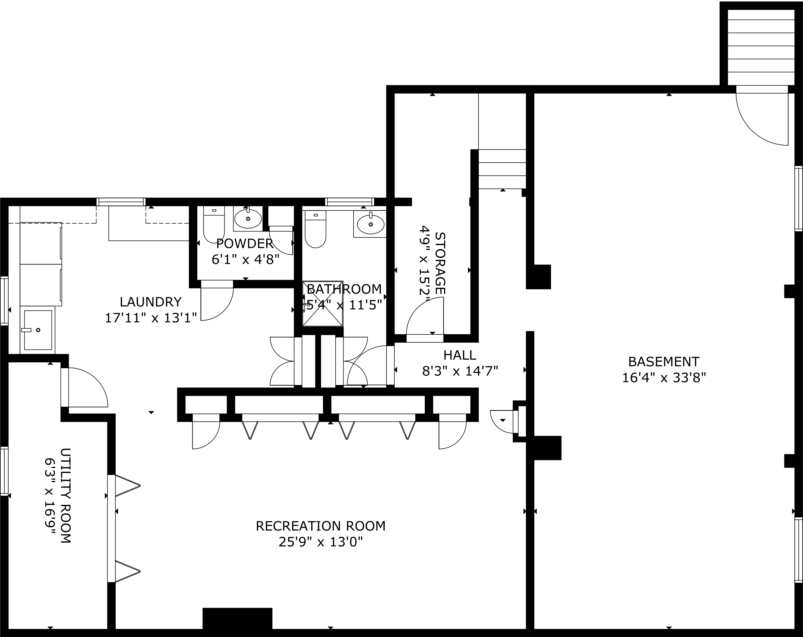
LOWER FLOOR
