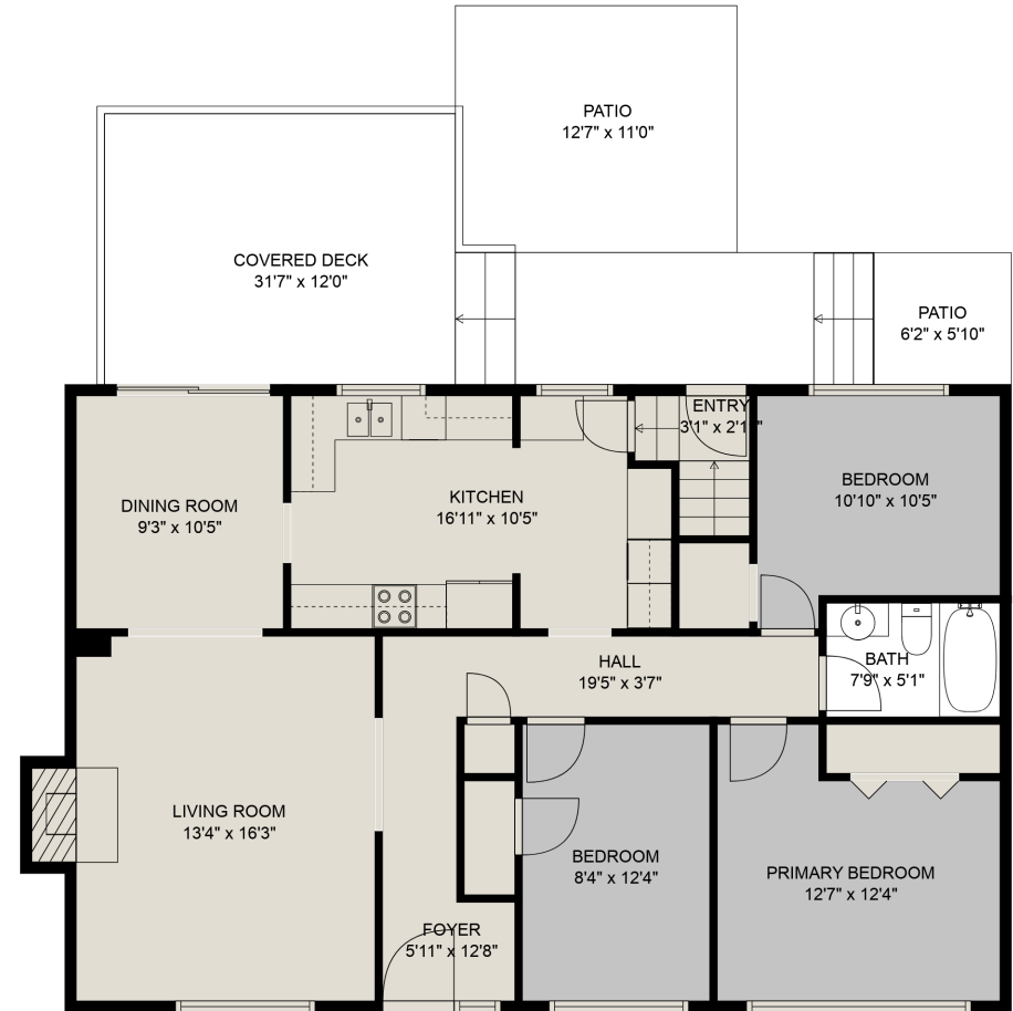
MAIN FLOOR
