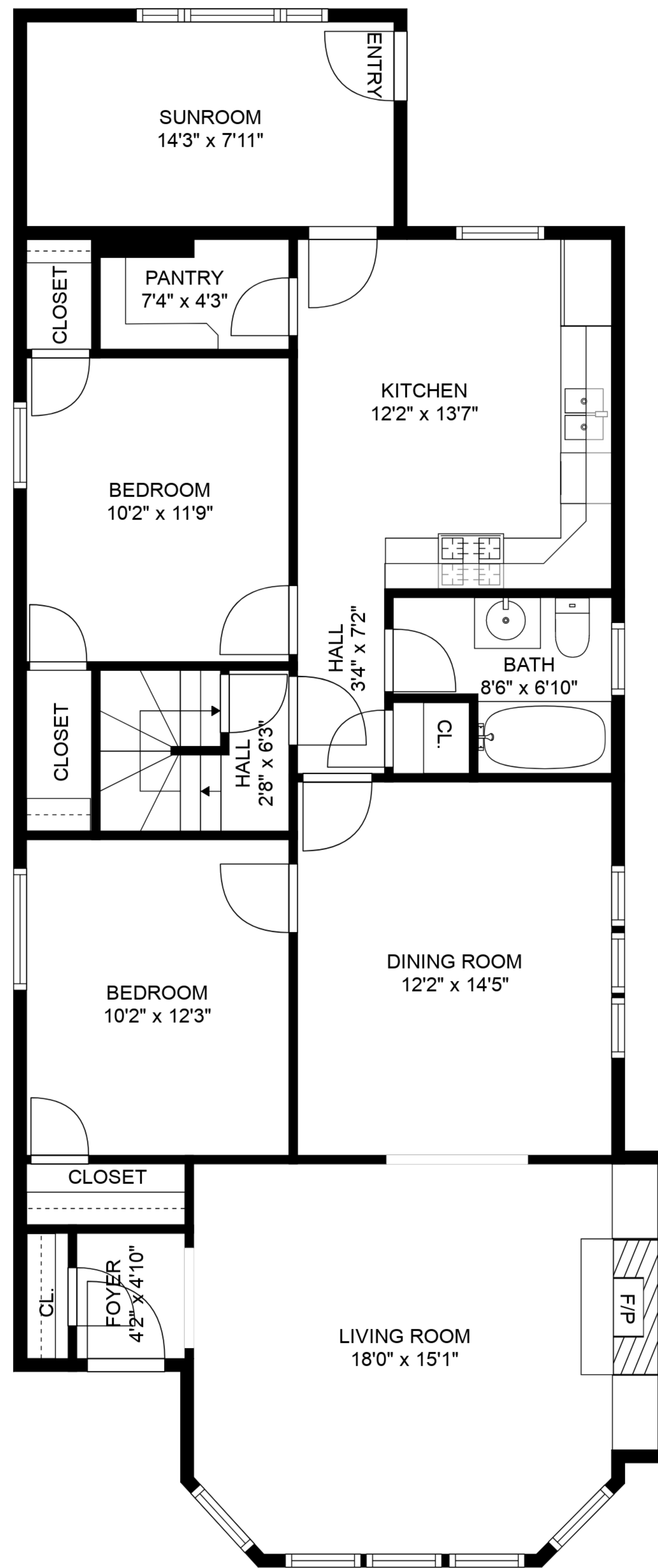
FLOOR 2
