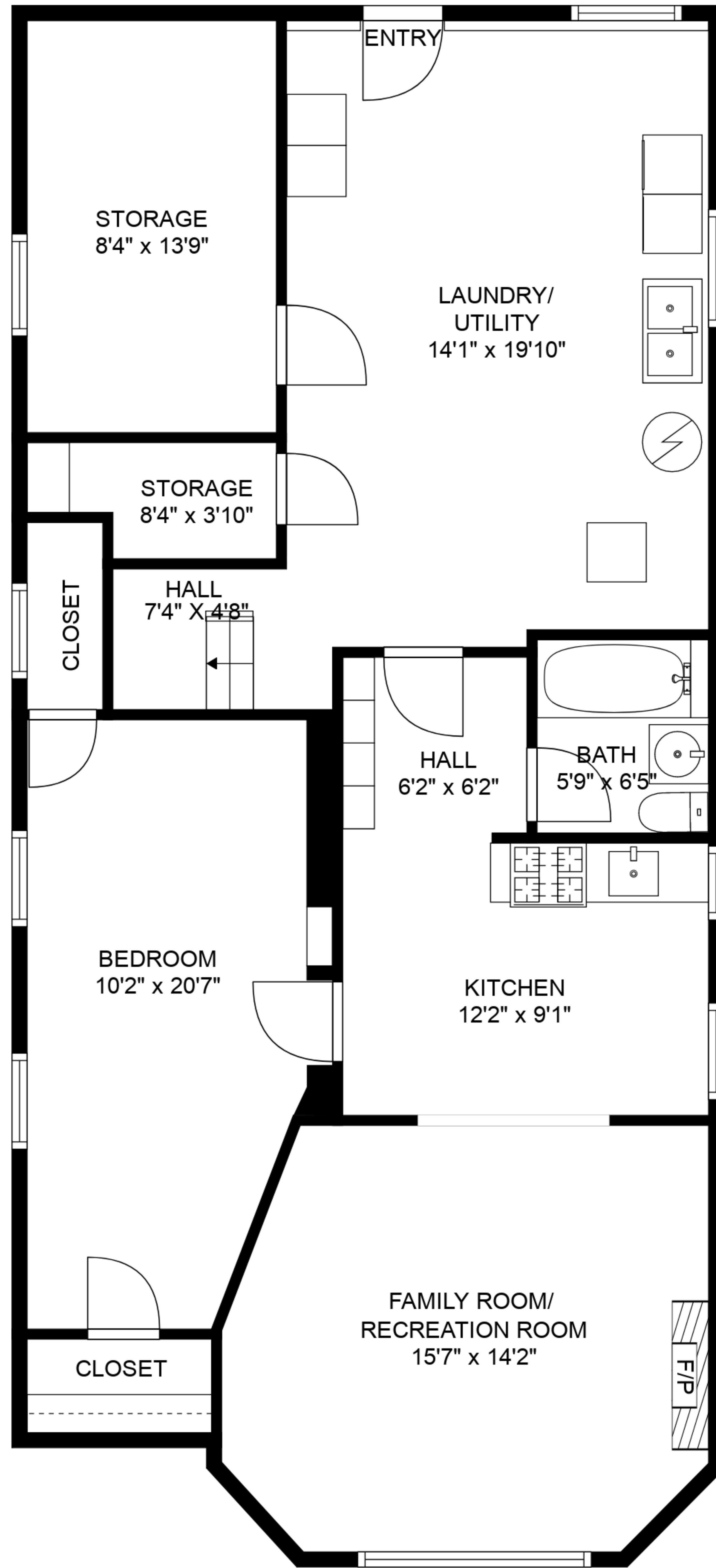
FLOOR 1
