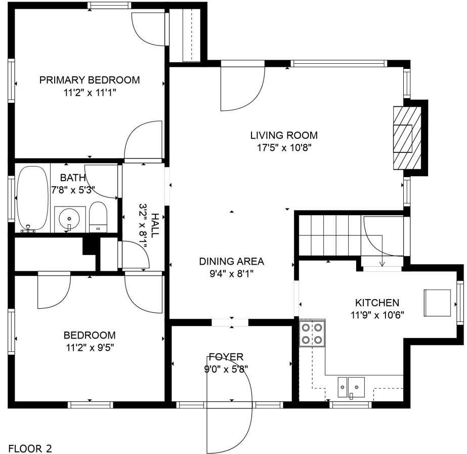
FLOOR 2
