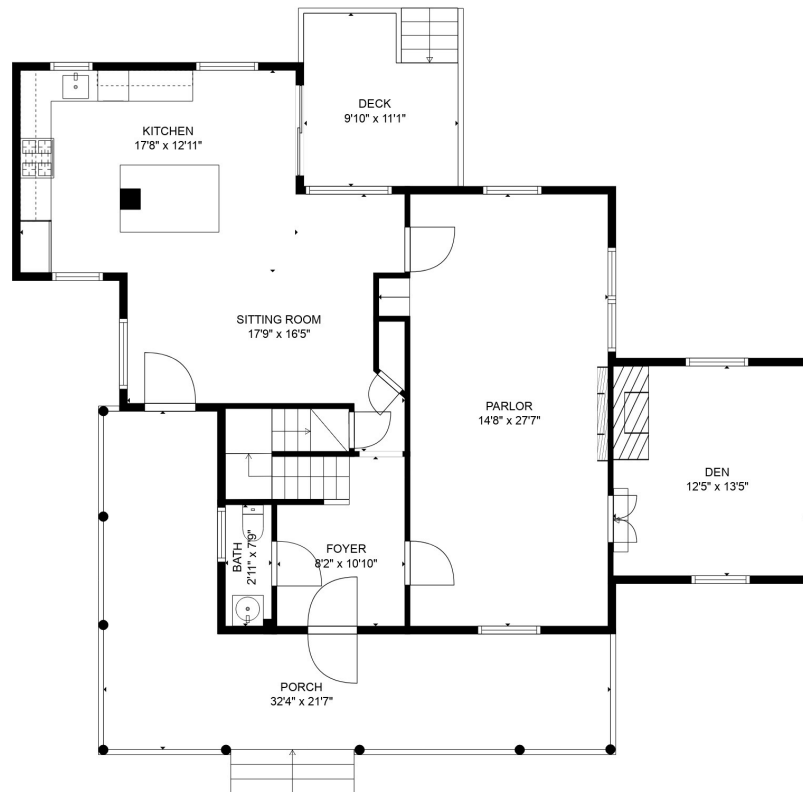
MAIN FLOOR
