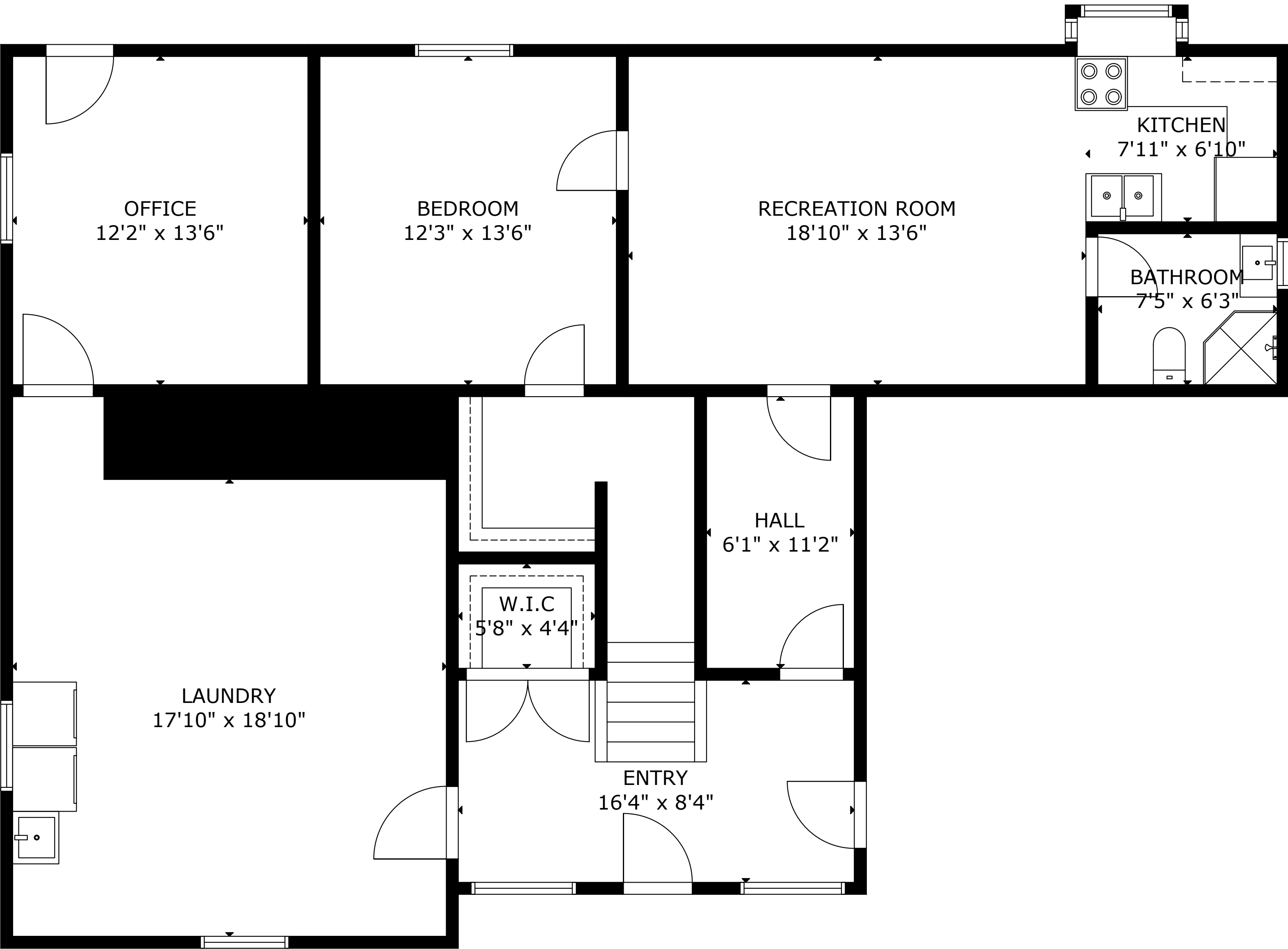
FLOOR 1
