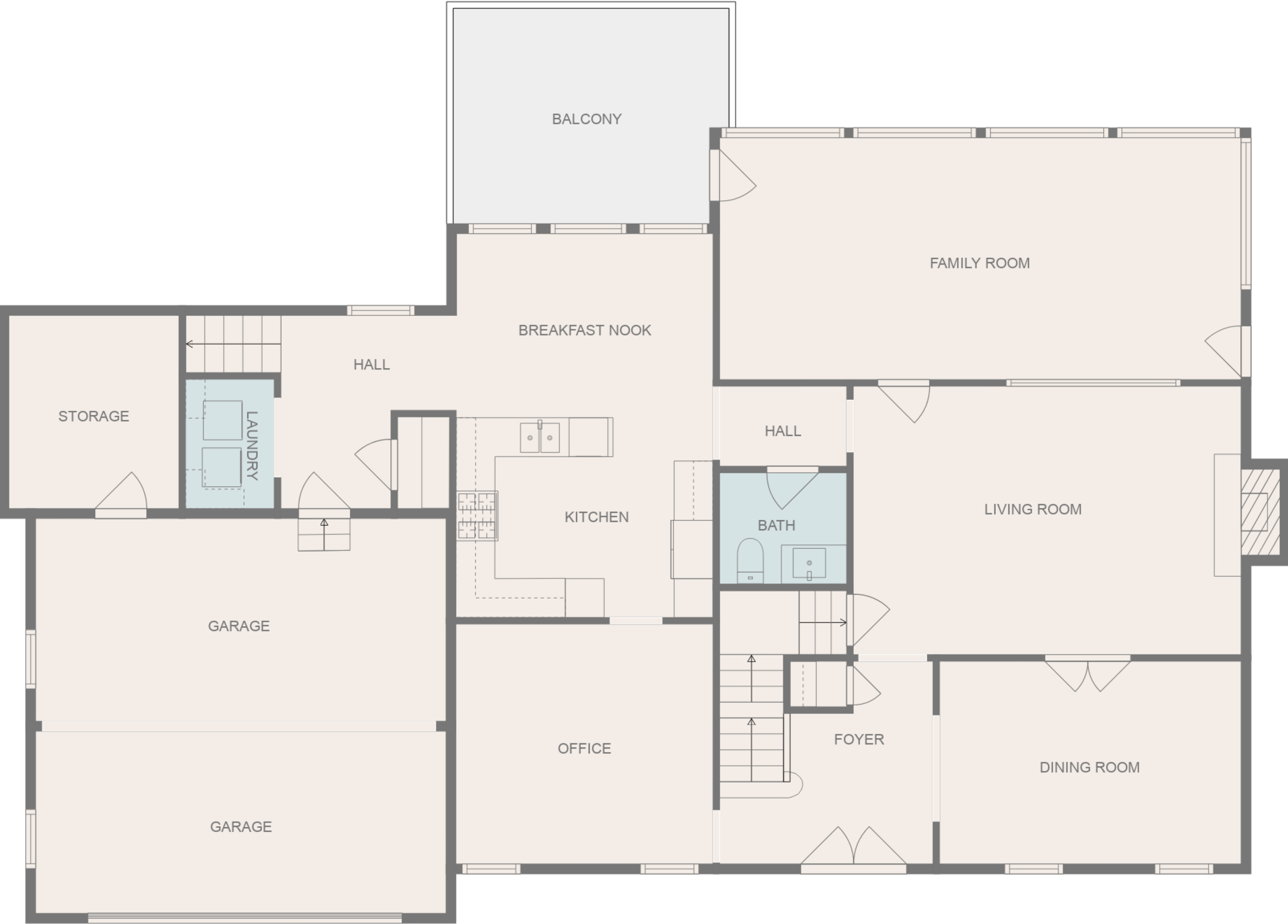
FLOOR 2
