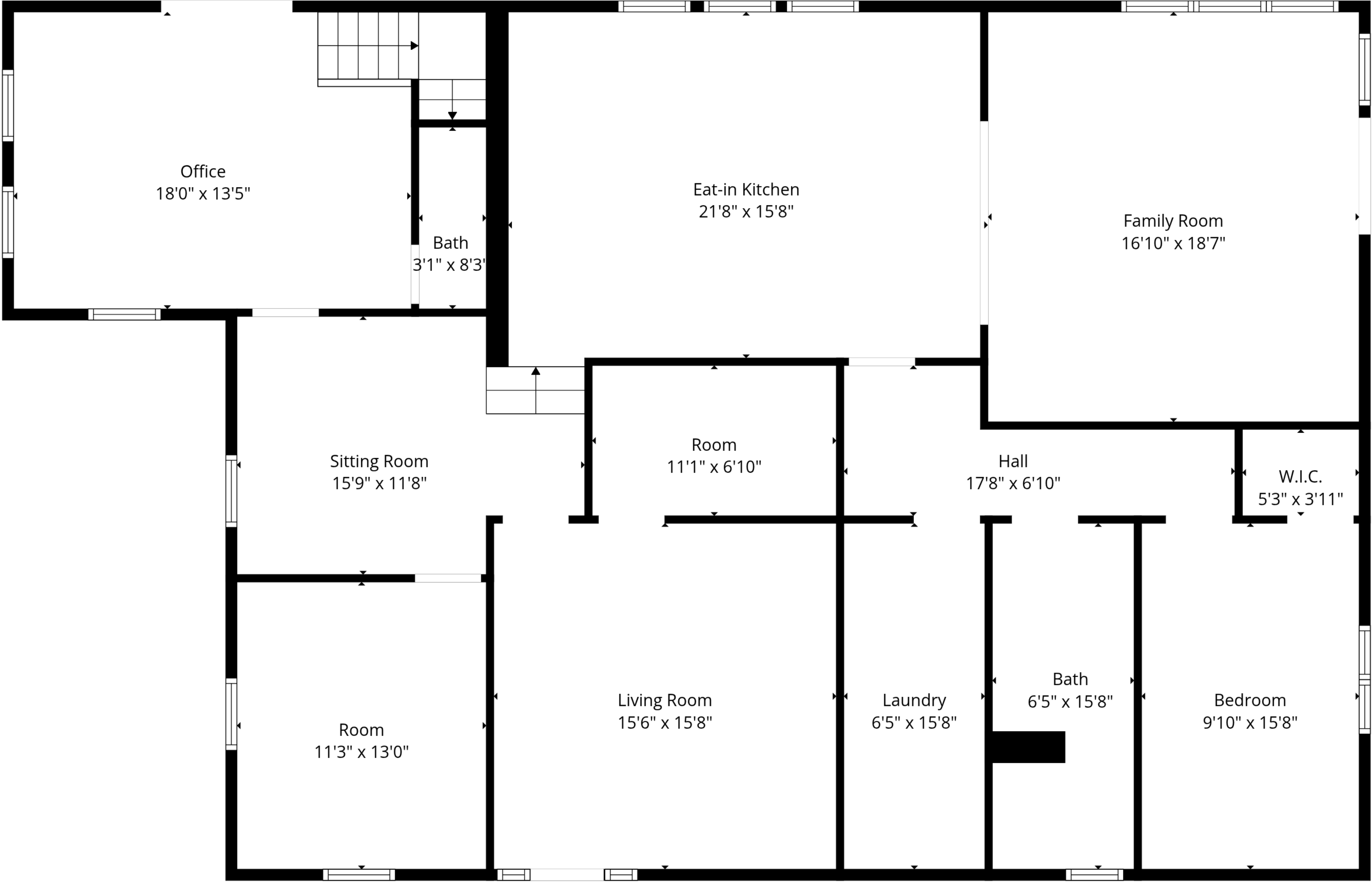
Floor 1
