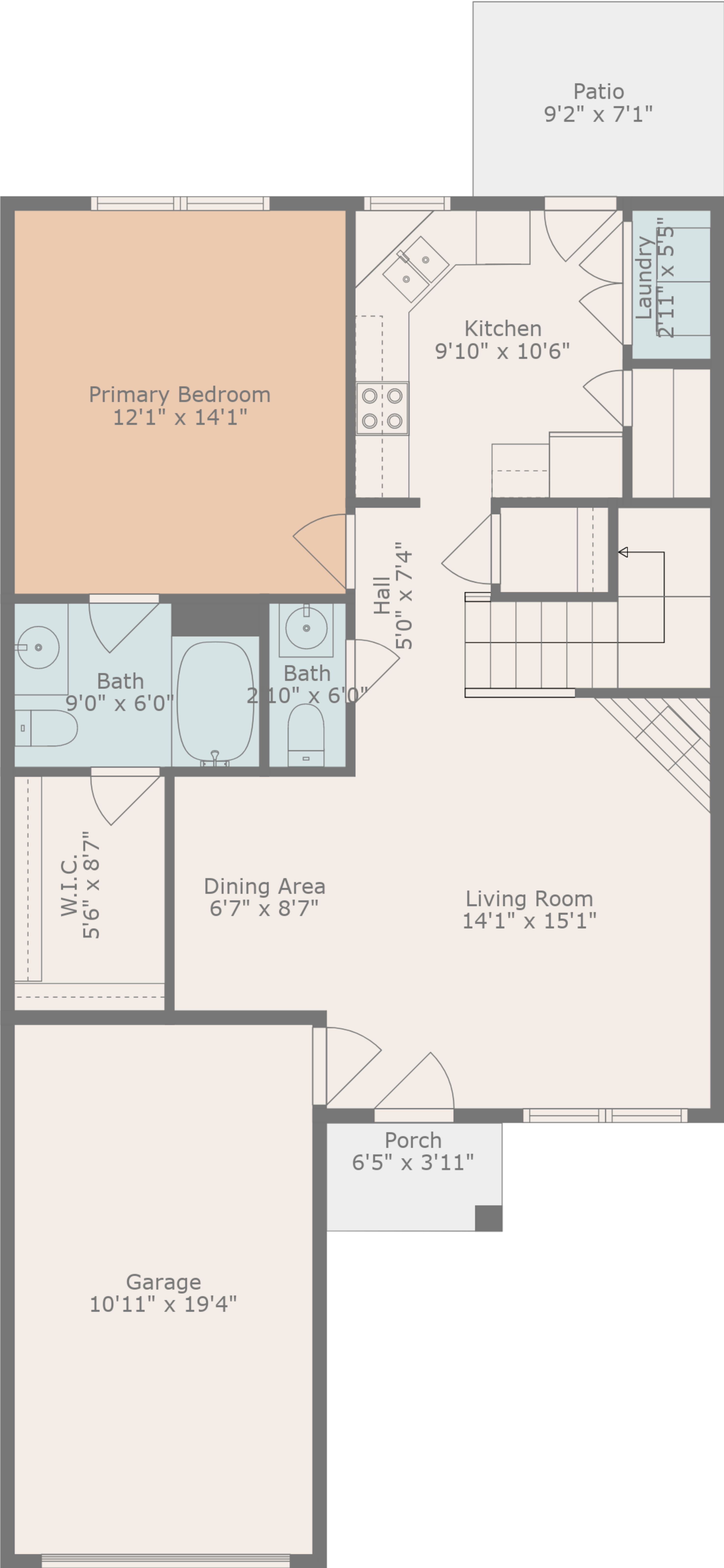
Floor 1
