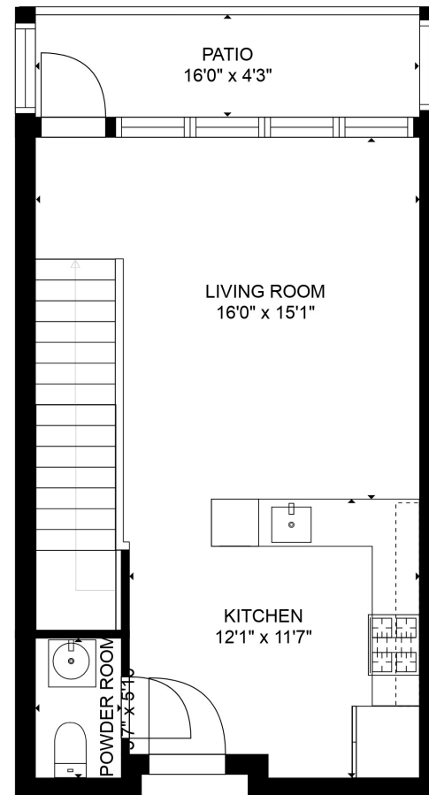
FLOOR 2
