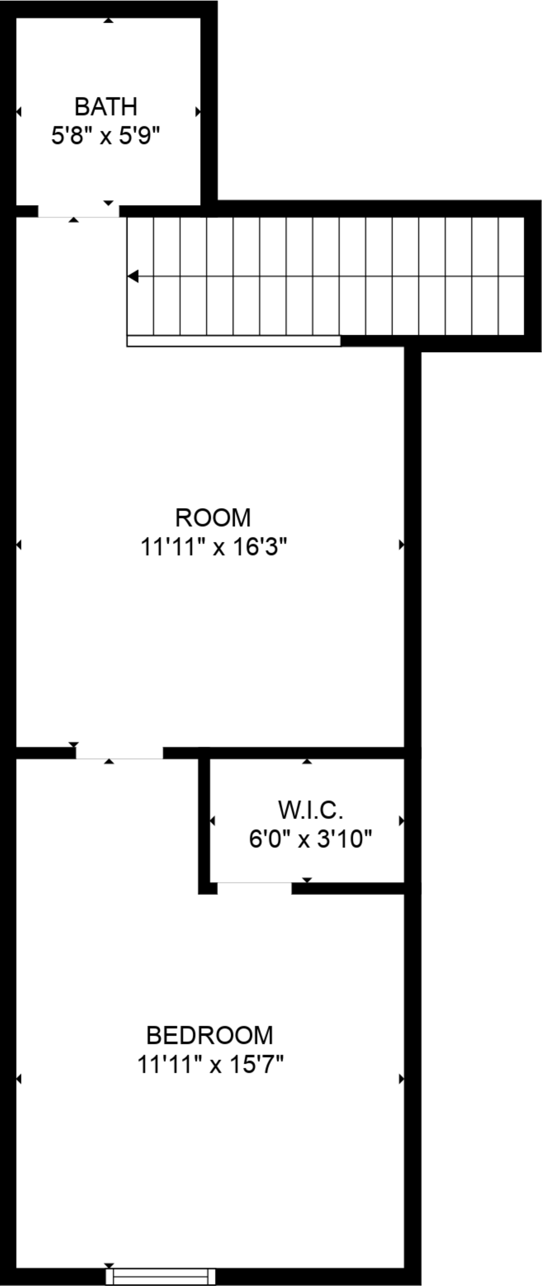
FLOOR 2
