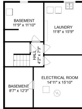
LOWER FLOOR
