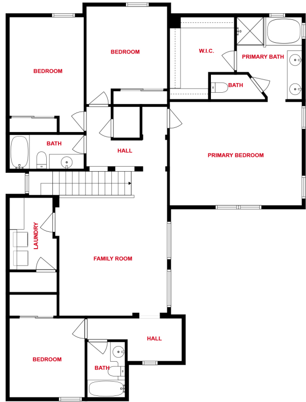
FLOOR 2
