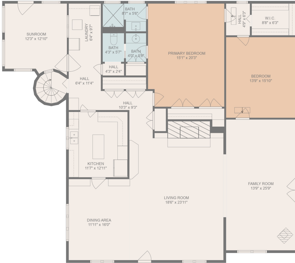
FLOOR 1
