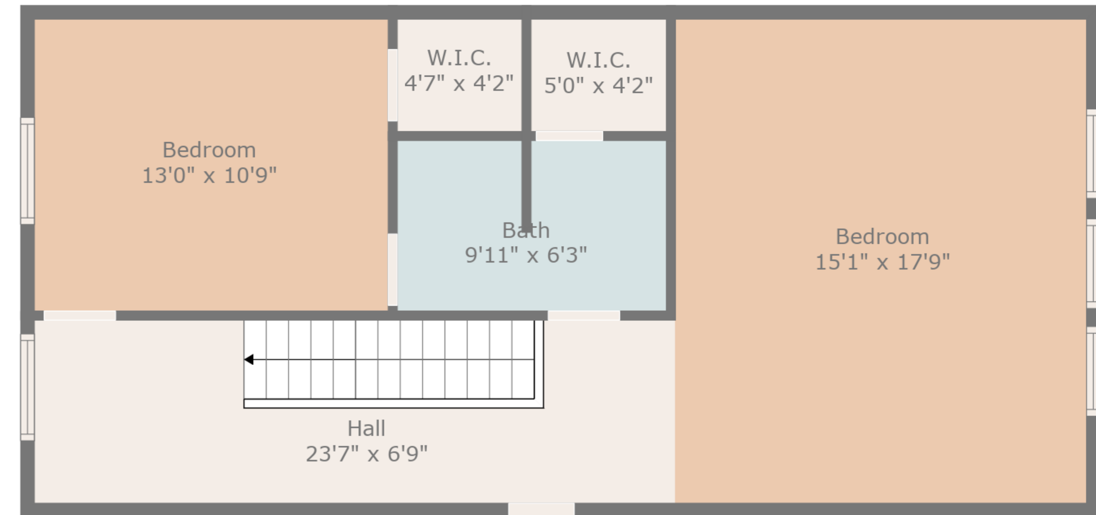
Floor 2
