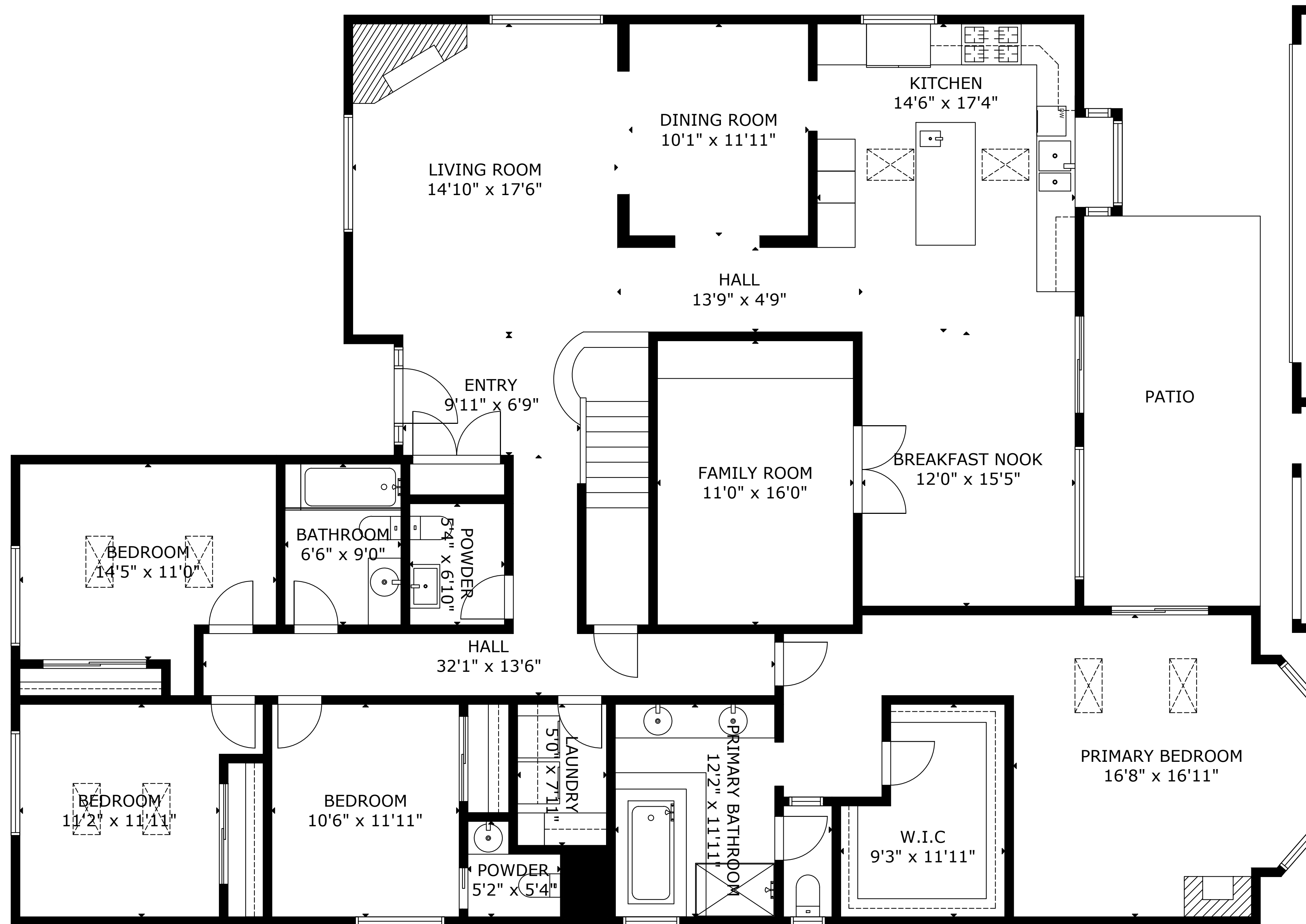
FLOOR 1
