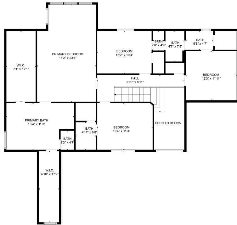
FLOOR 3
