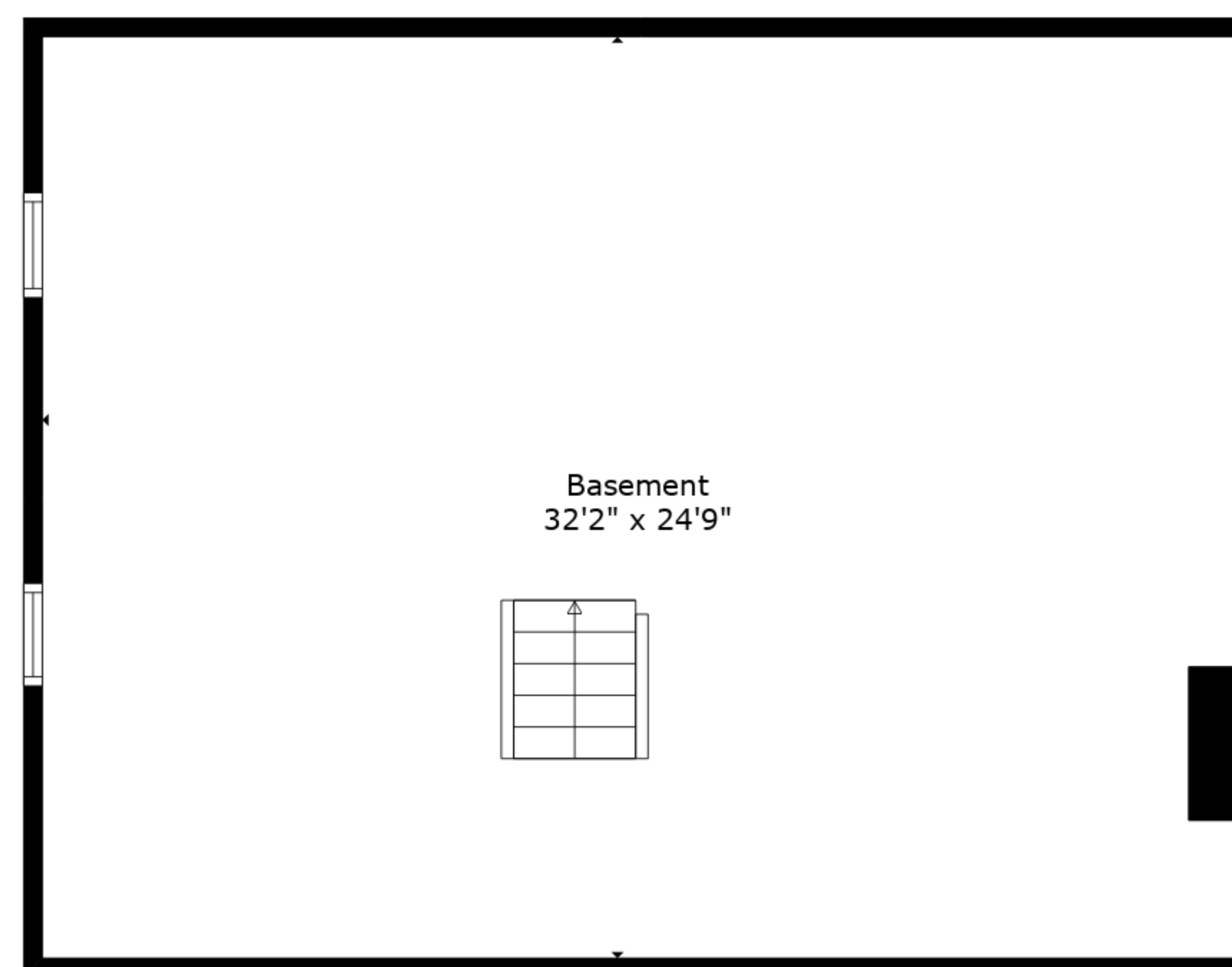
Floor 1
