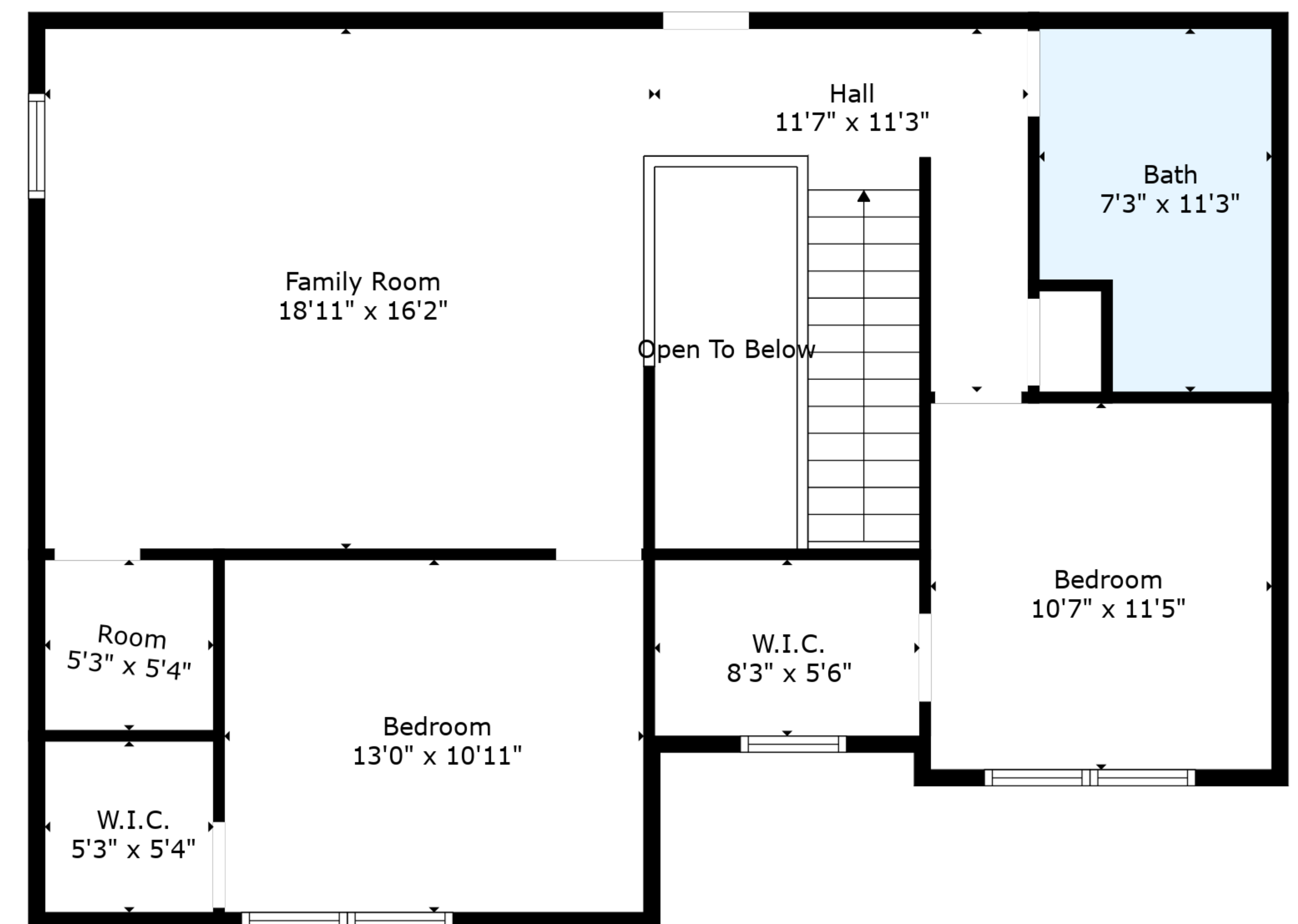
Floor 2
