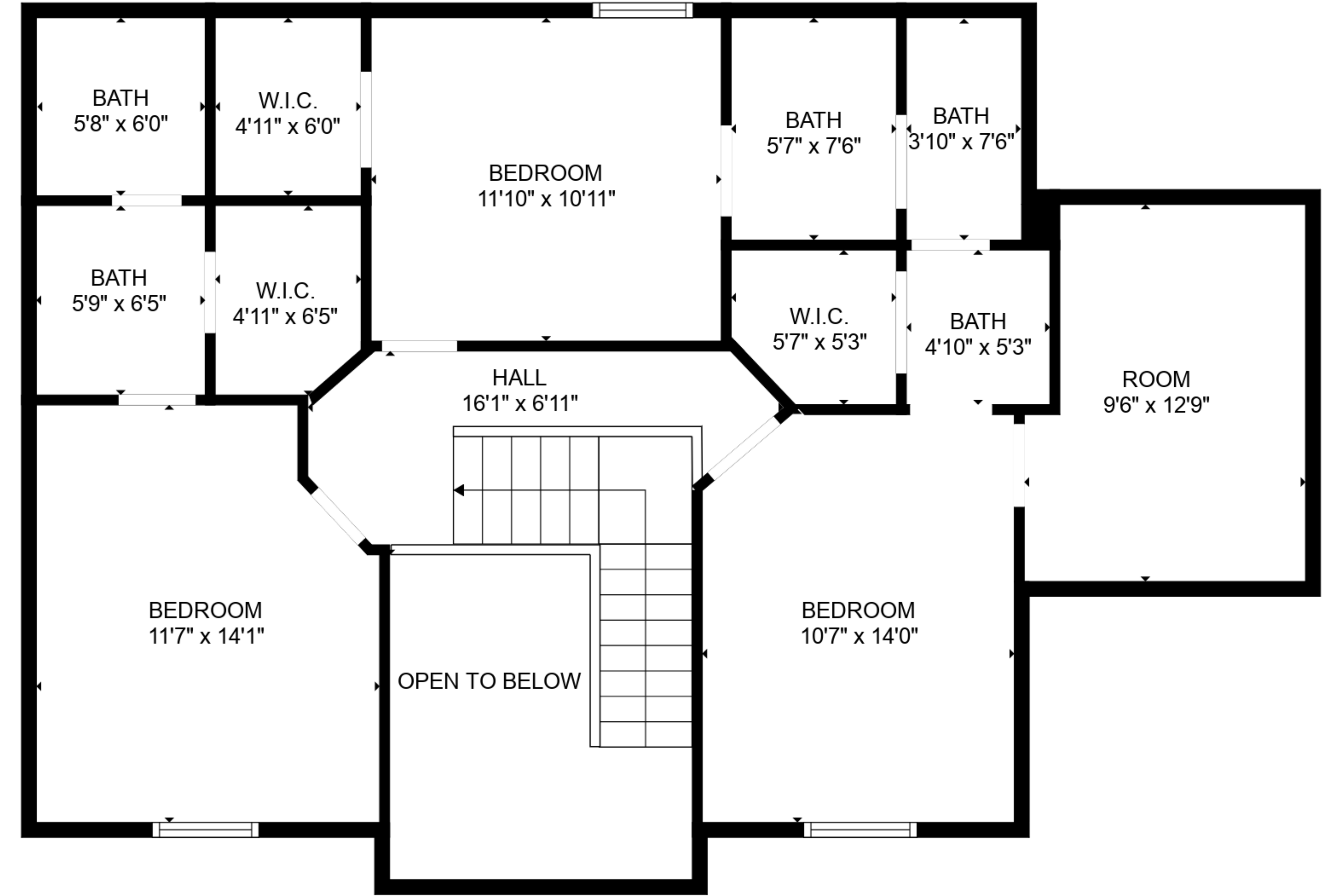
FLOOR 2
