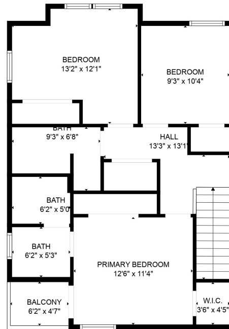
FLOOR 2
