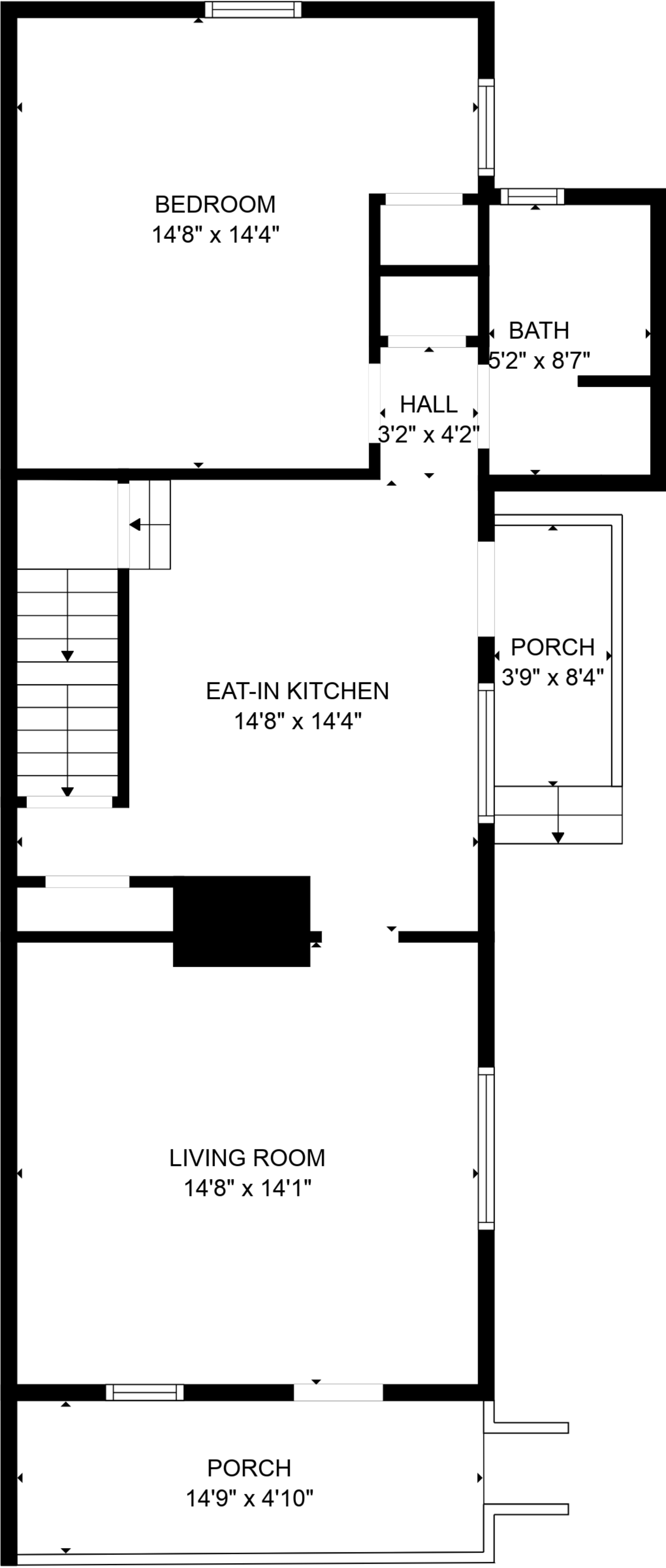
FLOOR 2
