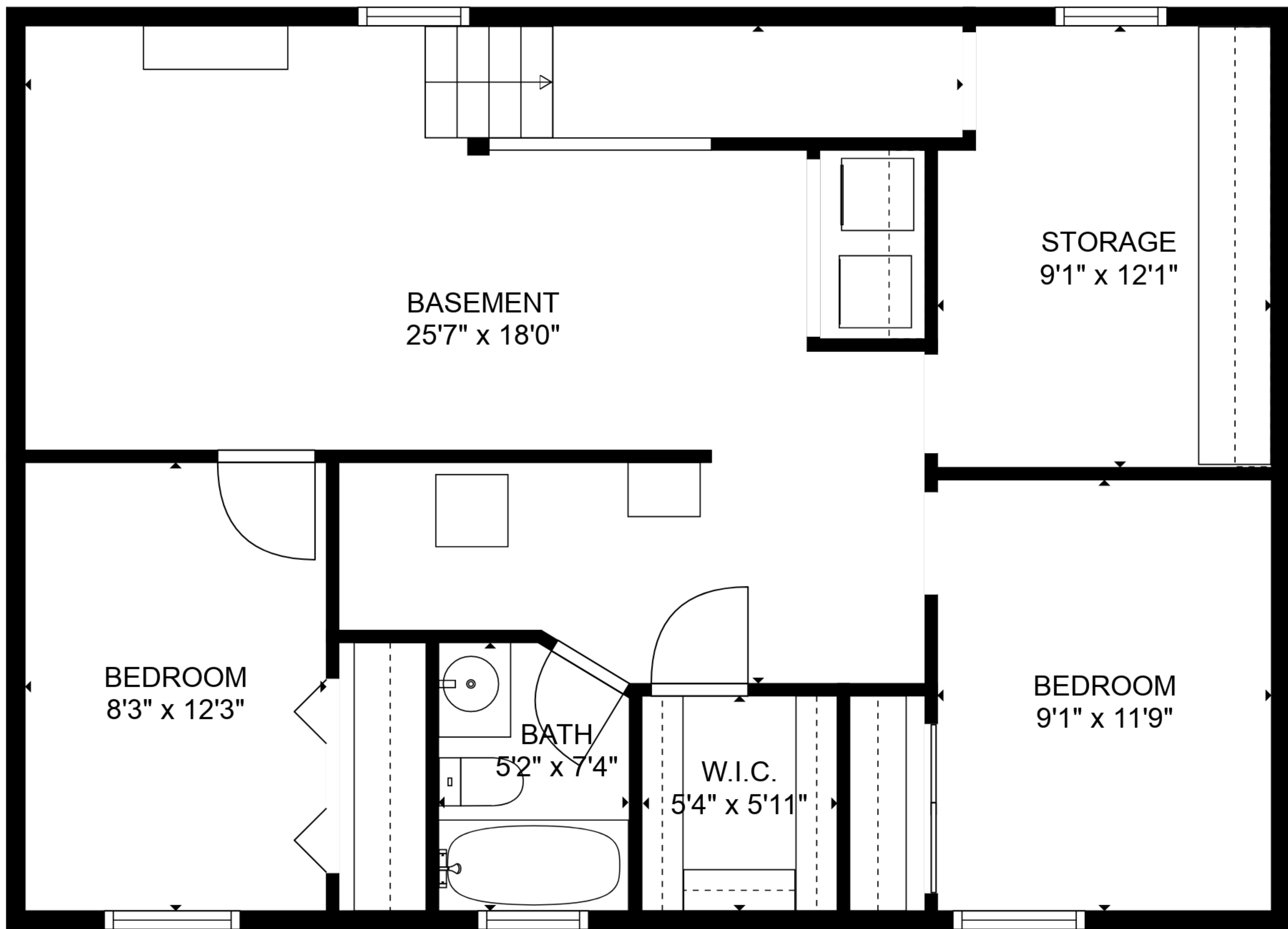
FLOOR 1
