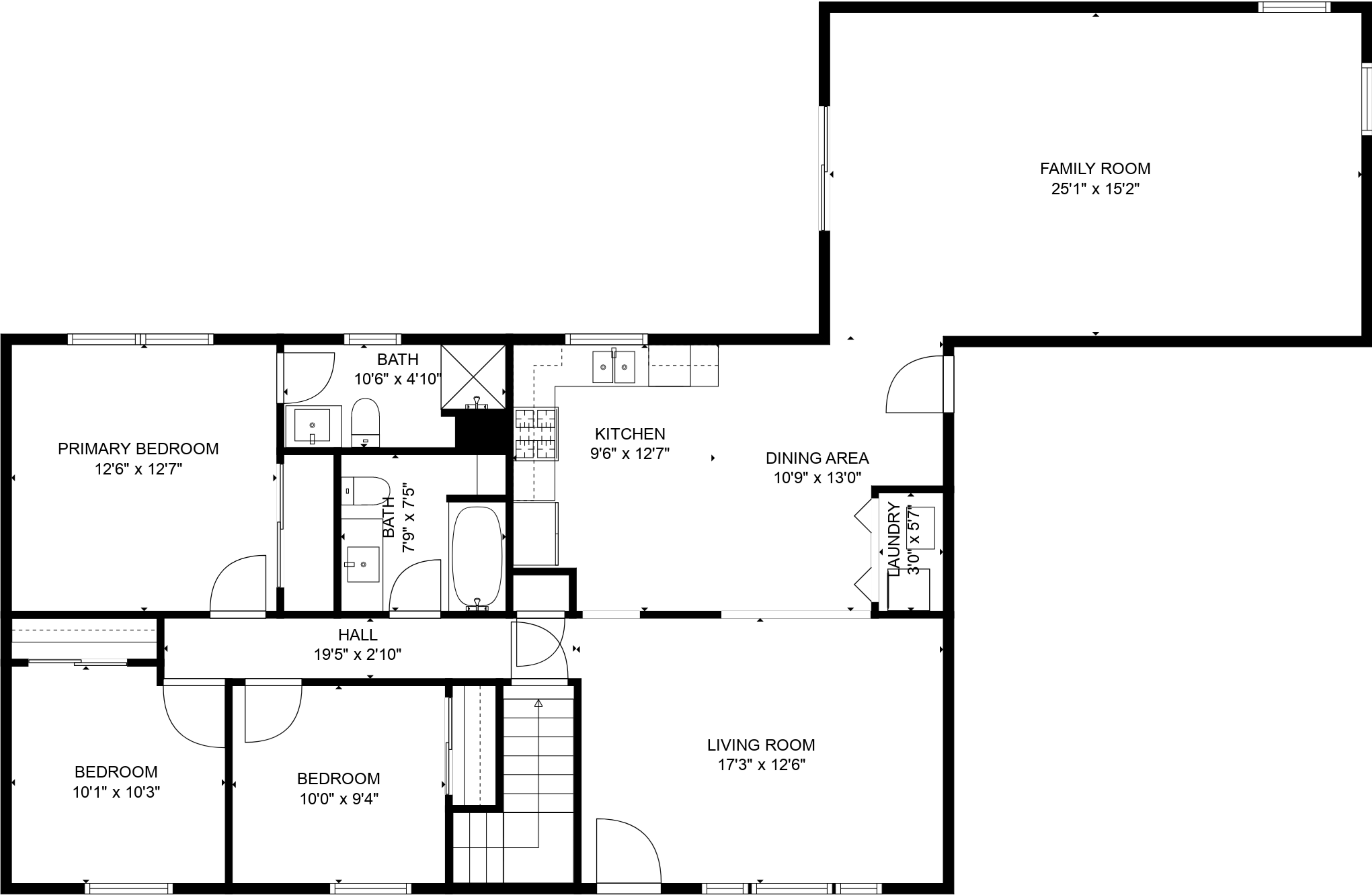
FLOOR 2
