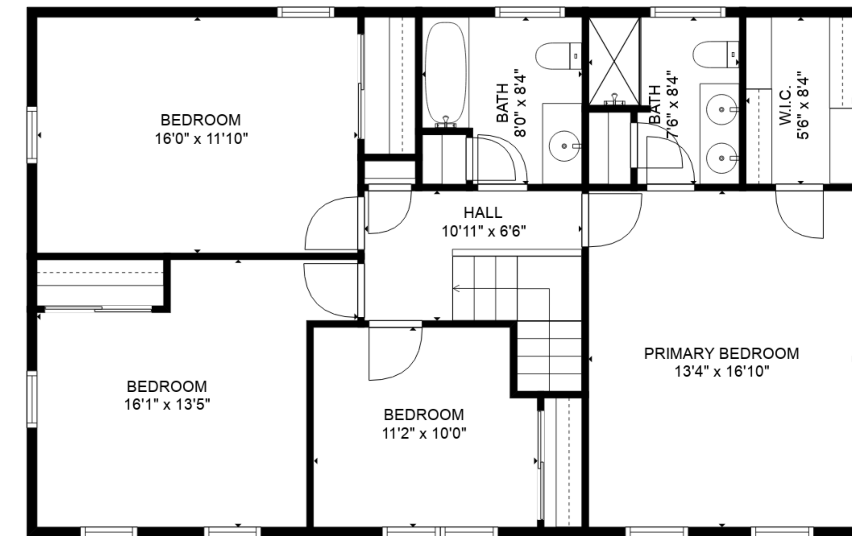
SECOND FLOOR
