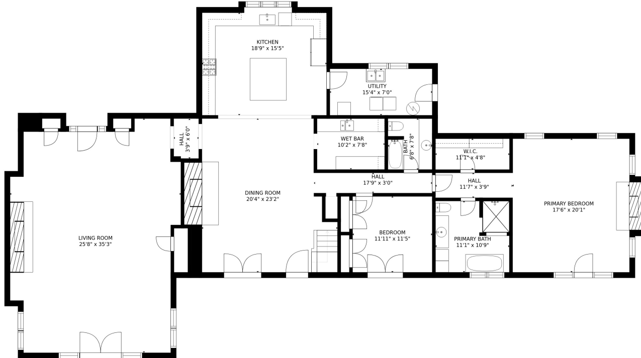
FLOOR 1
