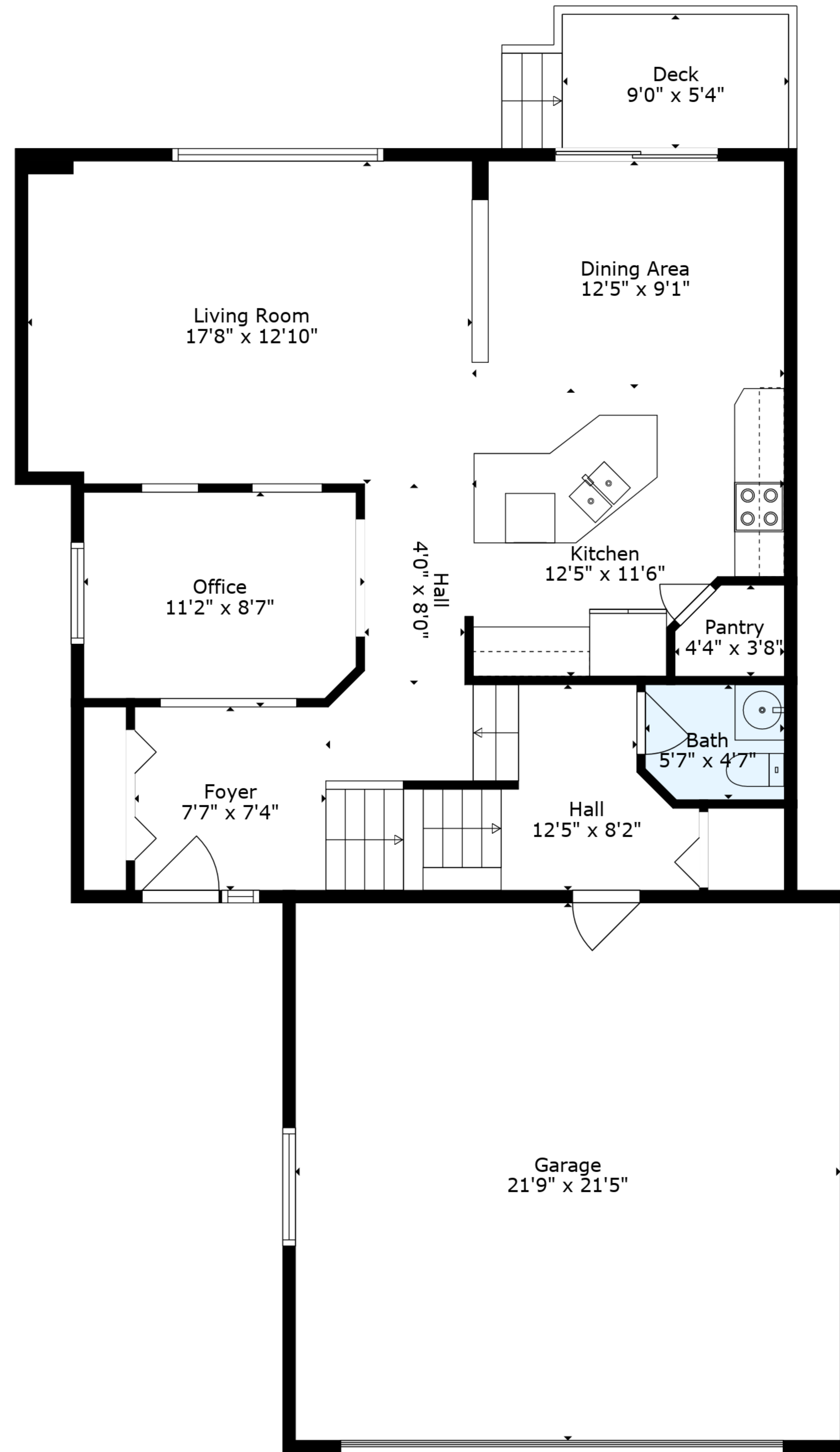
Floor 2
