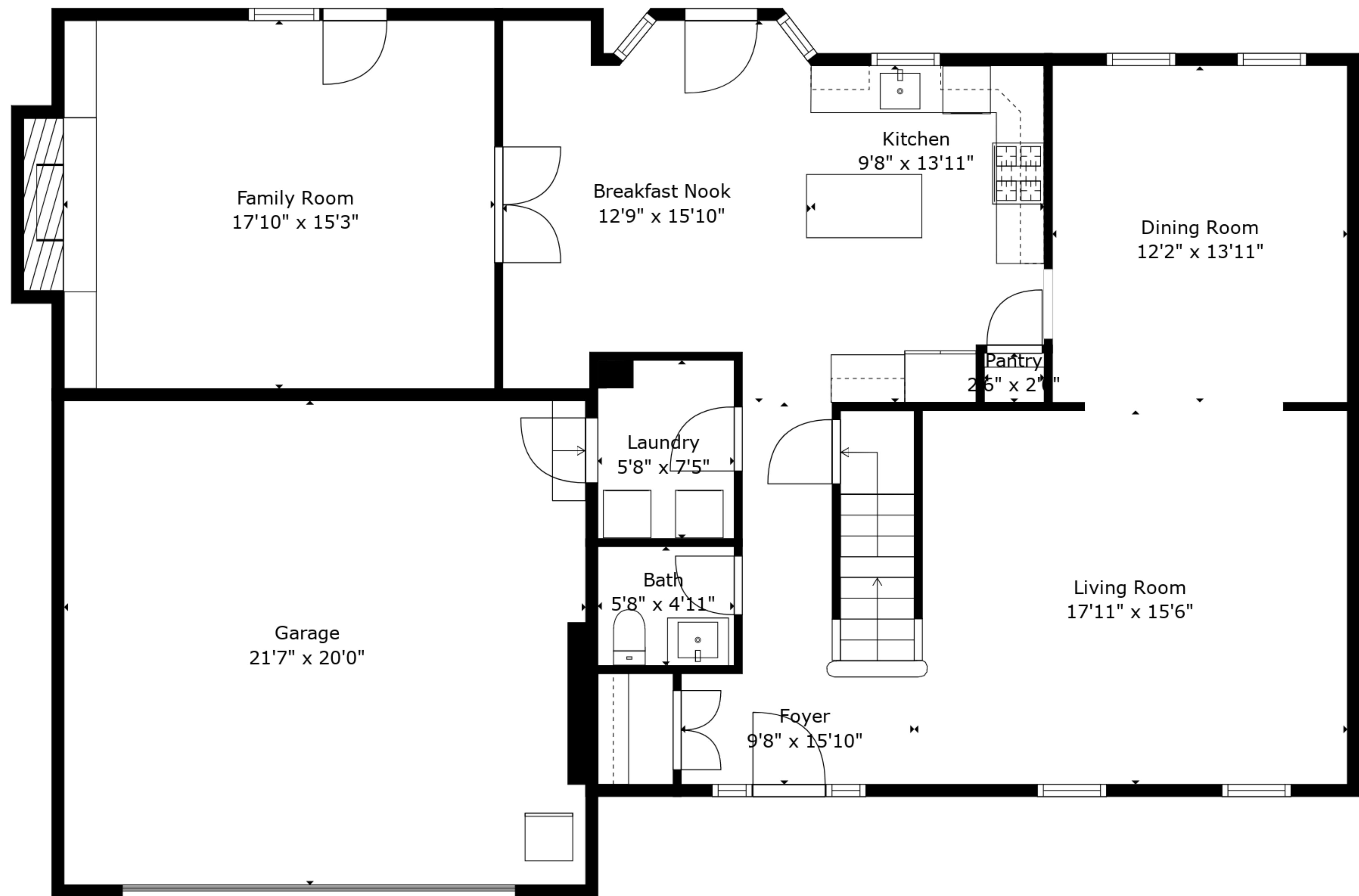
Floor 2
