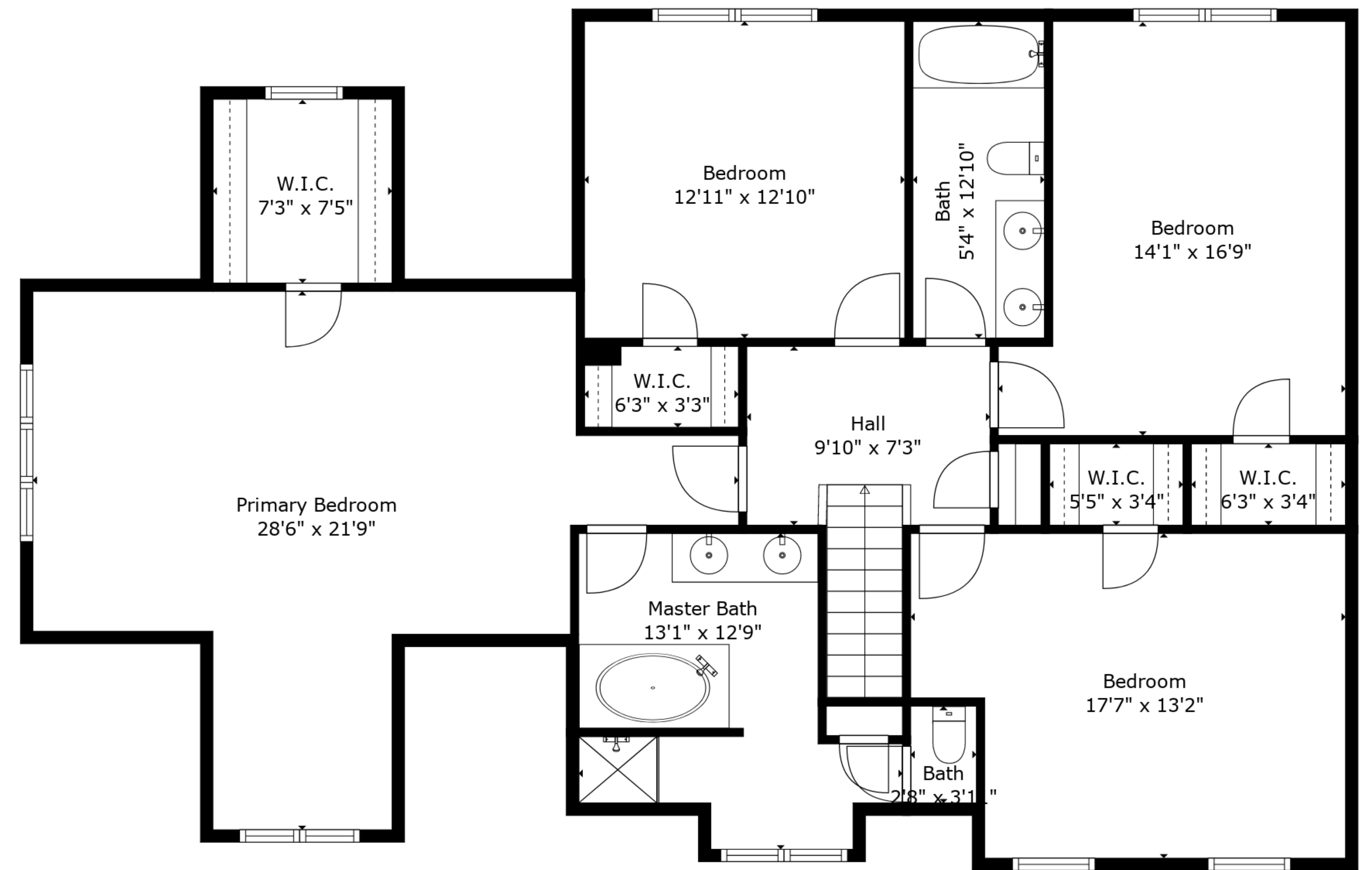
Floor 3
