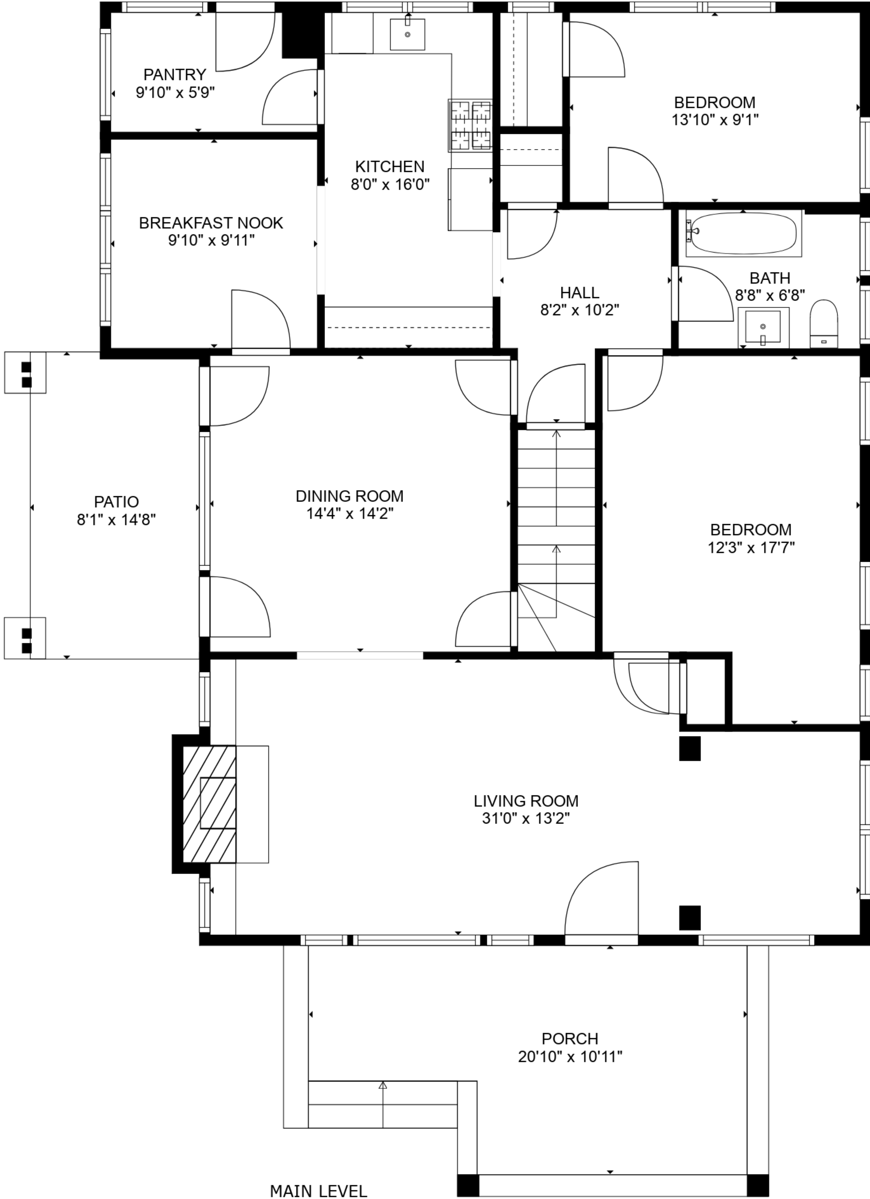
MAIN LEVEL
