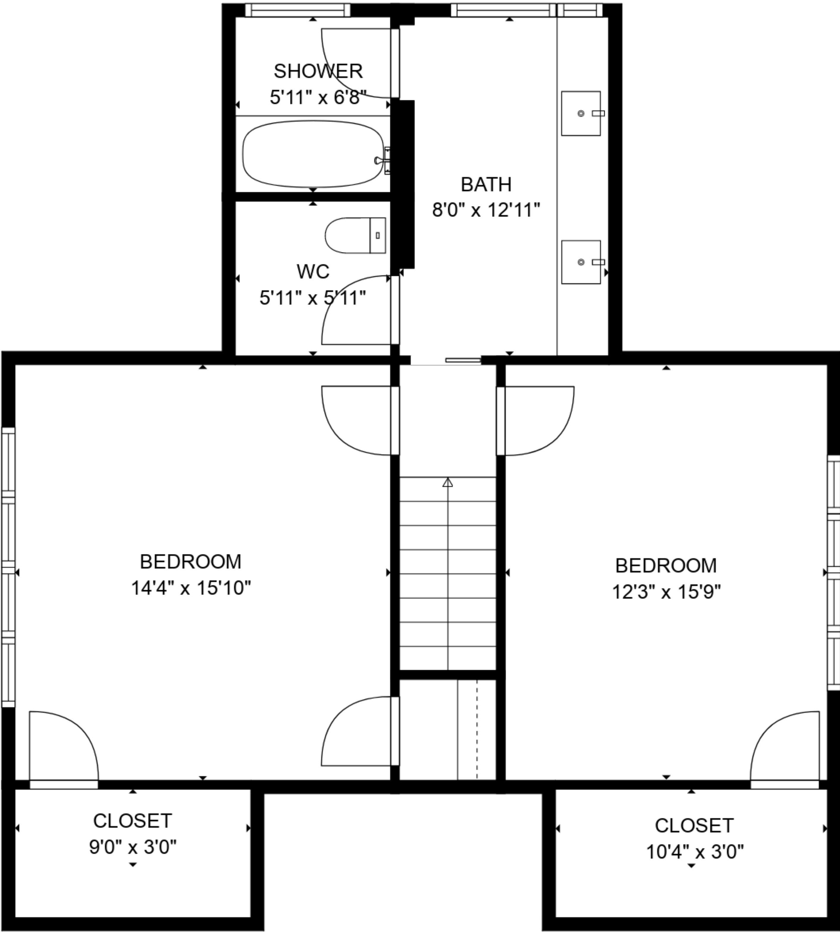
UPPER LEVEL
