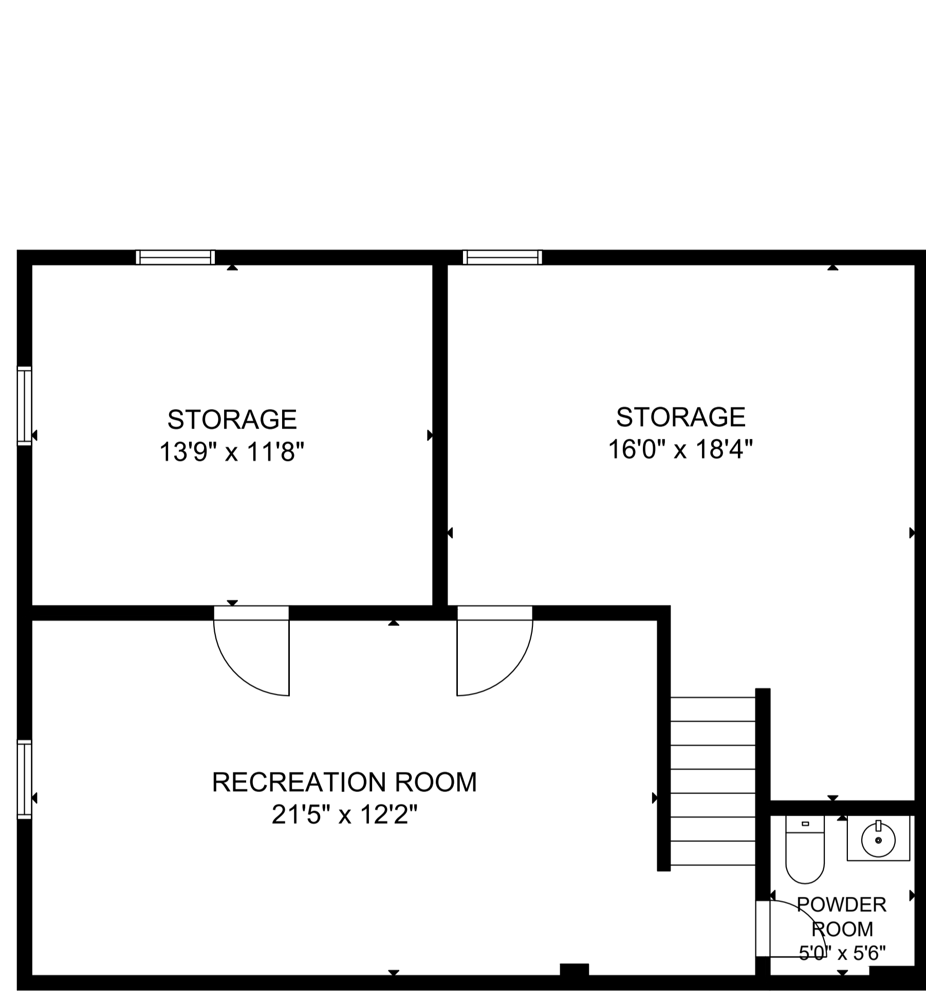
FLOOR 1
