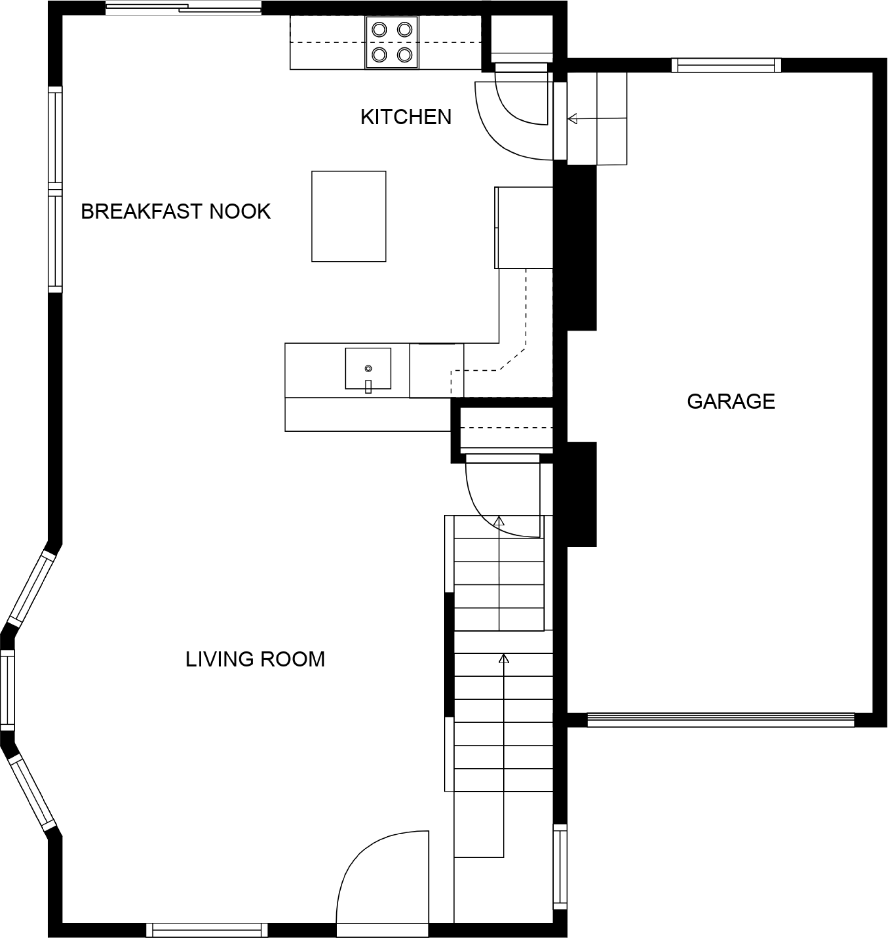
FLOOR 2
