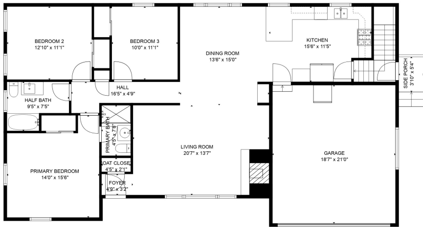
FLOOR 2
