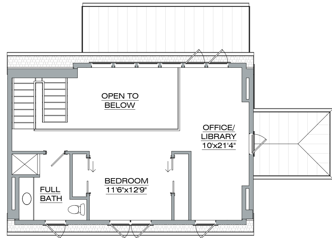
COTTAGE - SECOND FLOOR PLAN
