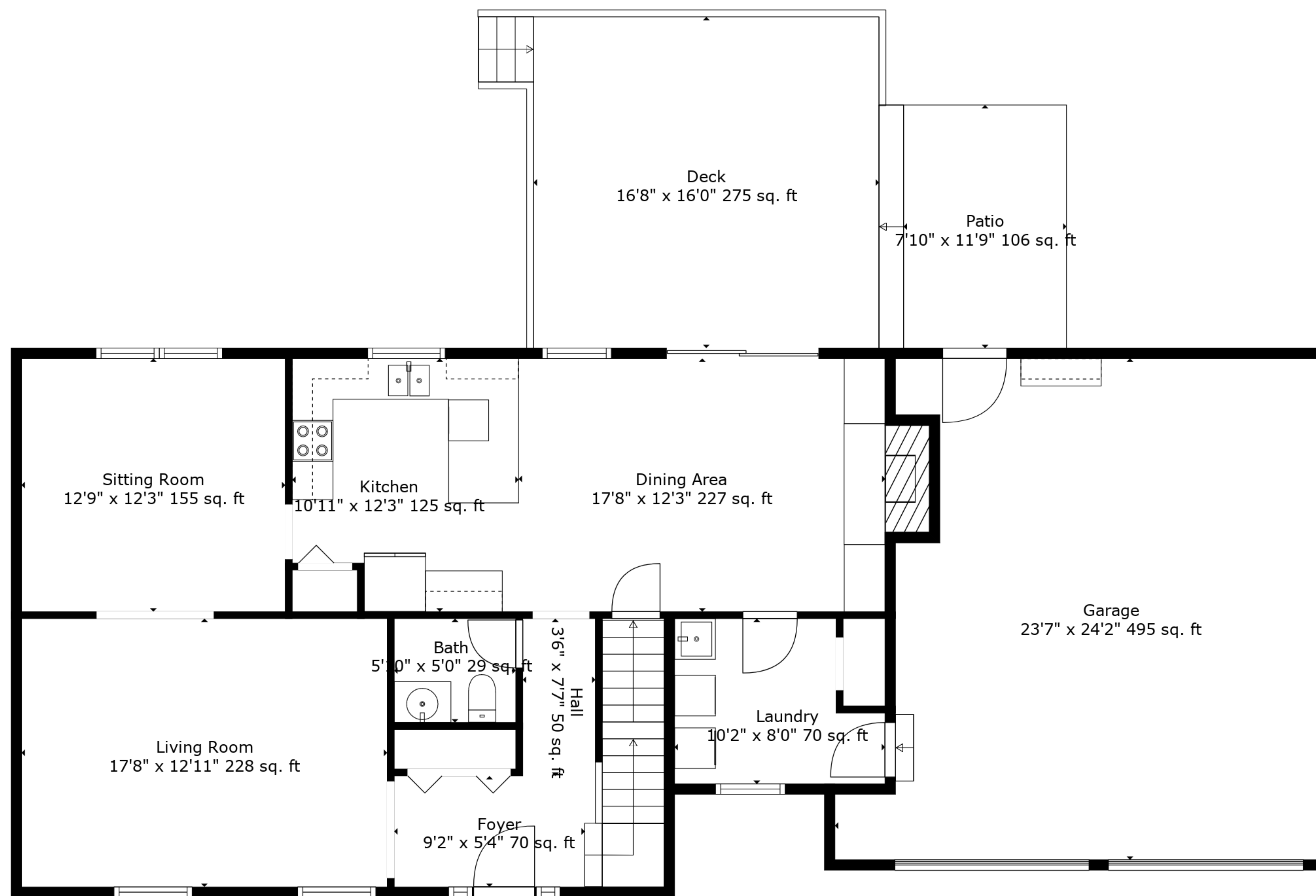
Floor 2
