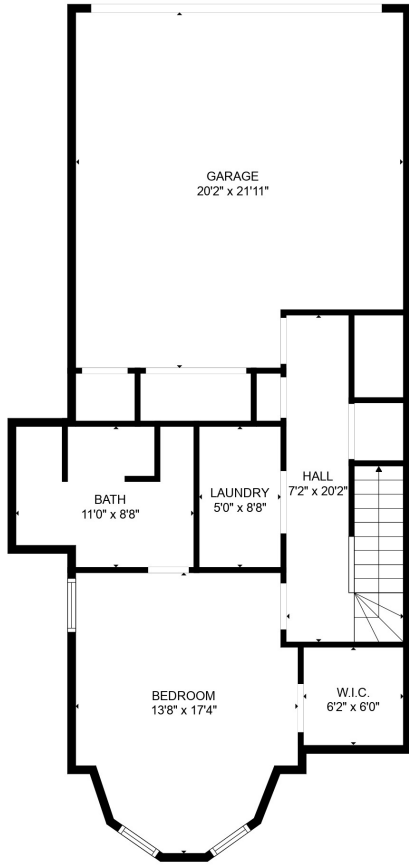
FLOOR 1
