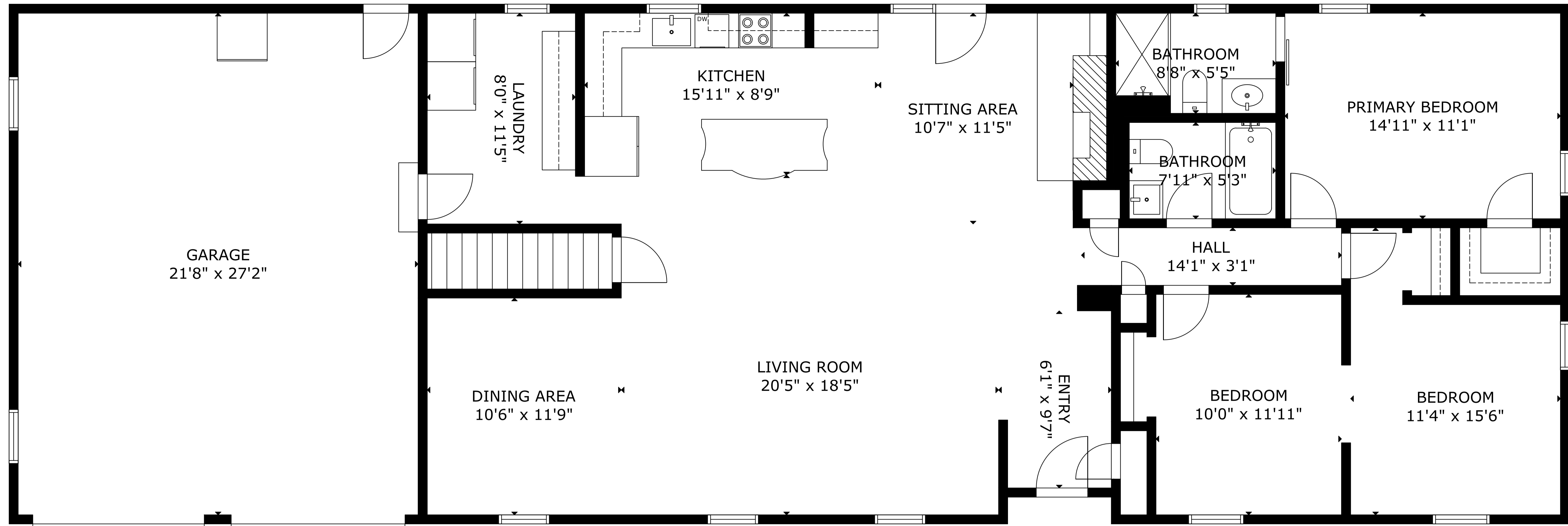
MAIN FLOOR
