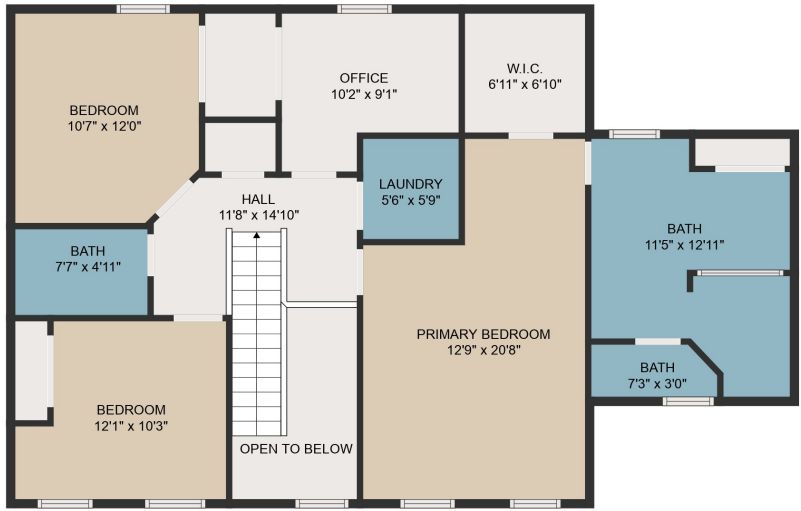
FLOOR 3
