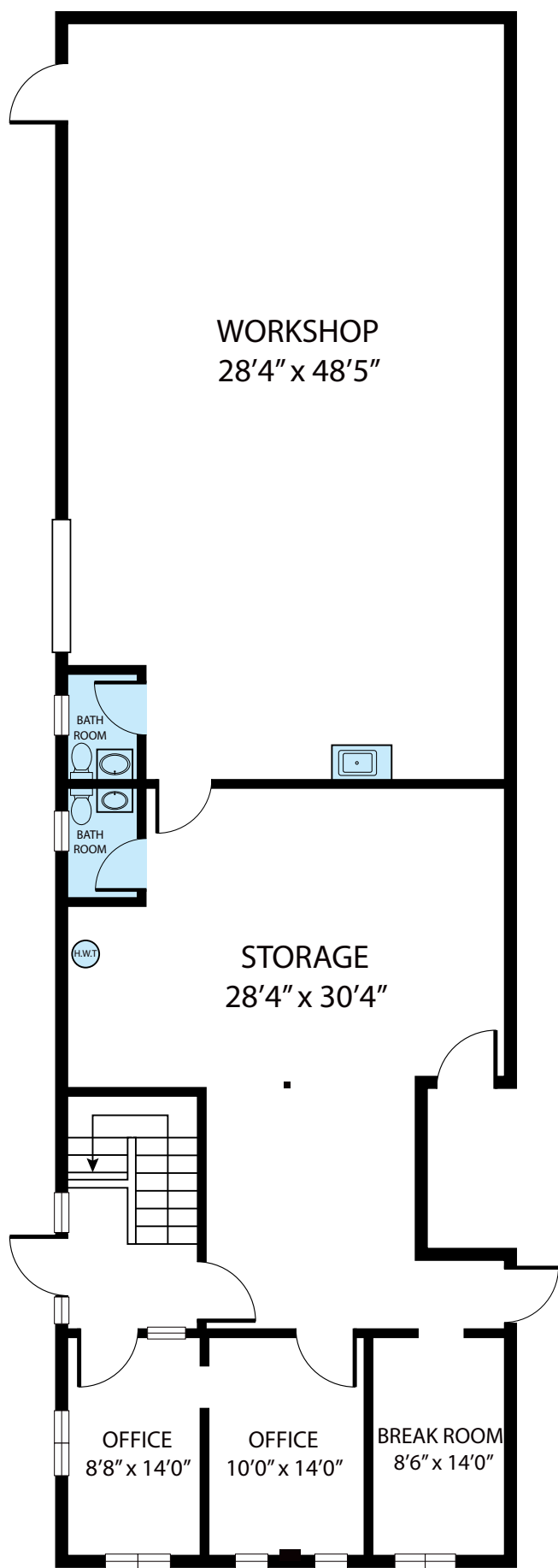
FIRST FLOOR
